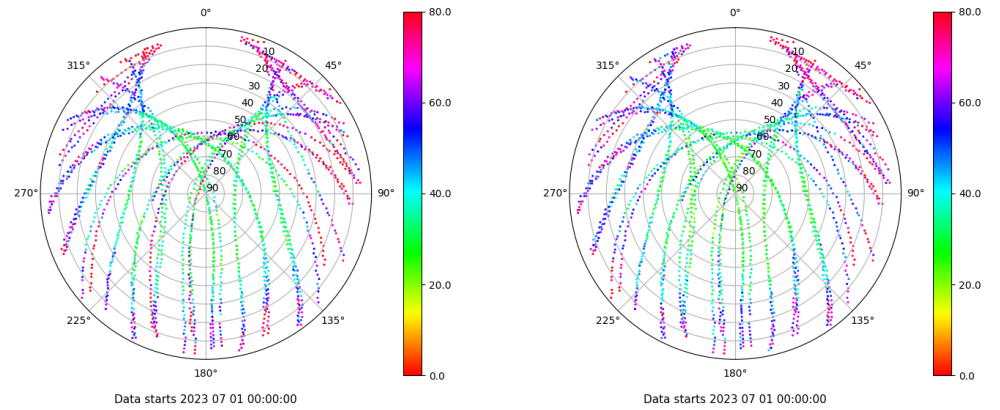
Skyplot for station BUIT. Parameter M1C Data file BUIT00ESP_R_2023182.xtr Skyplot for station BUIT. Parameter M2C Data file BUIT00ESP_R_2023182.xtr
