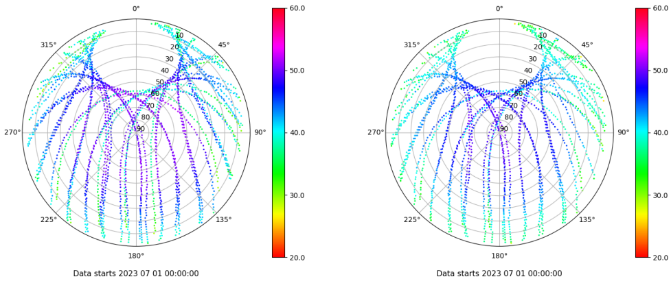
Skyplot for station BUIT. Signal to Noise S1C Data file BUIT00ESP_R_2023182.xtr Skyplot for station BUIT. Signal to Noise S2C Data file BUIT00ESP_R_2023182.xtr
