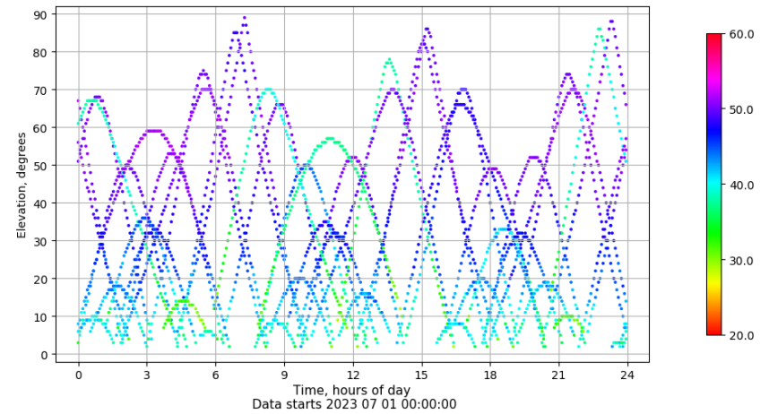
Time-elevation plot for station BUIT. Signal to Noise S1C Data file BUIT00ESP_R_2023182.xtr
