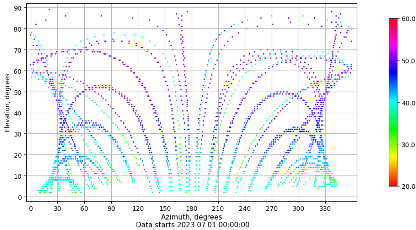
Azimuth-elevation plot for station BUIT. Signal to Noise S1C Data file BUIT00ESP_R_2023182.xtr
