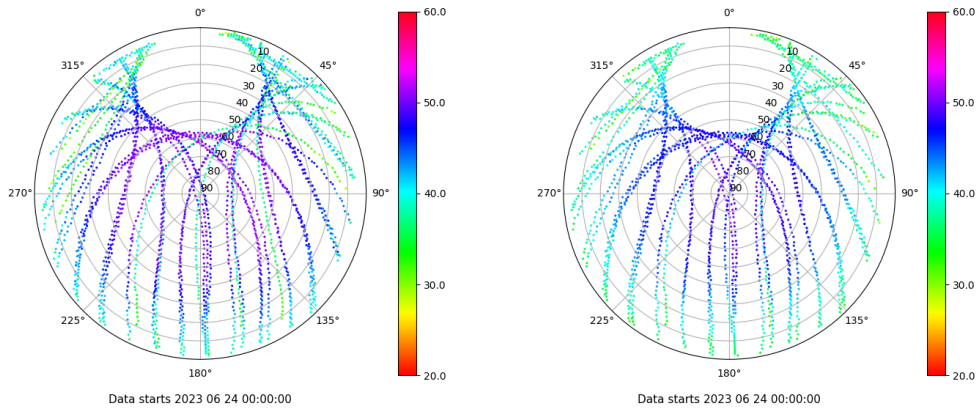
Skyplot for station BUIT. Signal to Noise S1C Data file BUIT00ESP_R_2023175.xtr Skyplot for station BUIT. Signal to Noise S2C Data file BUIT00ESP_R_2023175.xtr
