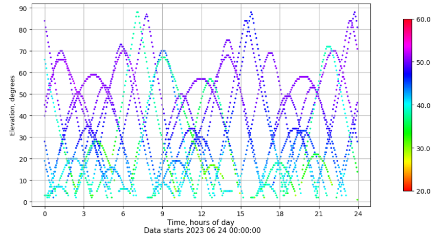
Time-elevation plot for station BUIT. Signal to Noise S1C Data file BUIT00ESP_R_2023175.xtr
