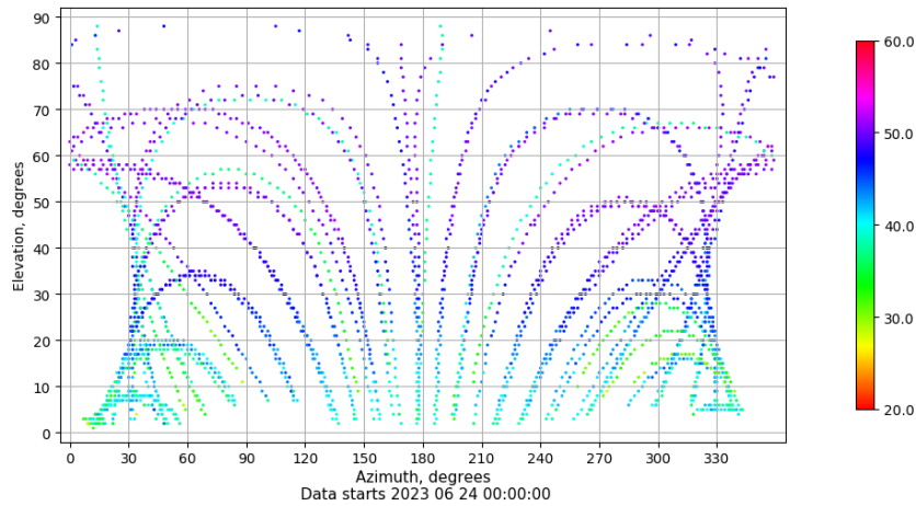
Azimuth-elevation plot for station BUIT. Signal to Noise S1C Data file BUIT00ESP_R_2023175.xtr
