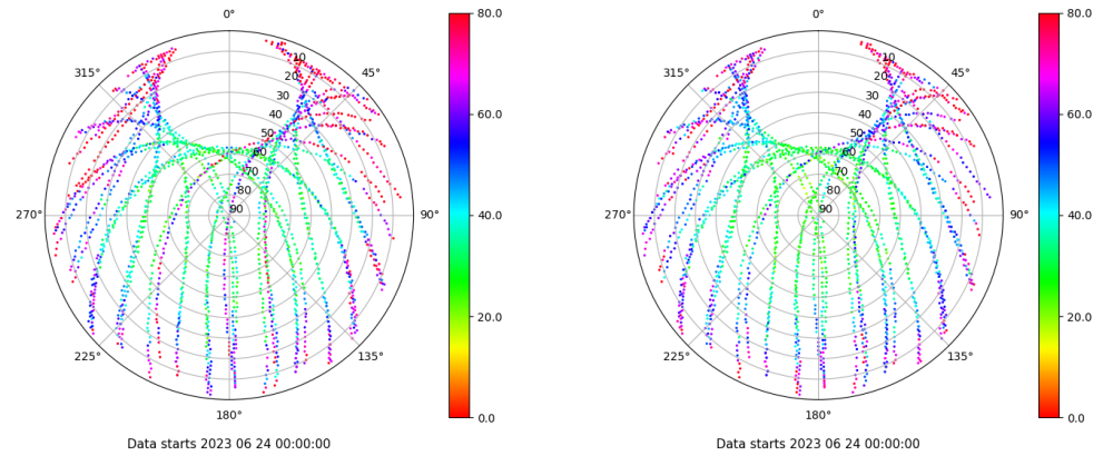
Skyplot for station BUIT. Parameter M1C Data file BUIT00ESP_R_2023175.xtr Skyplot for station BUIT. Parameter M2C Data file BUIT00ESP_R_2023175.xtr
