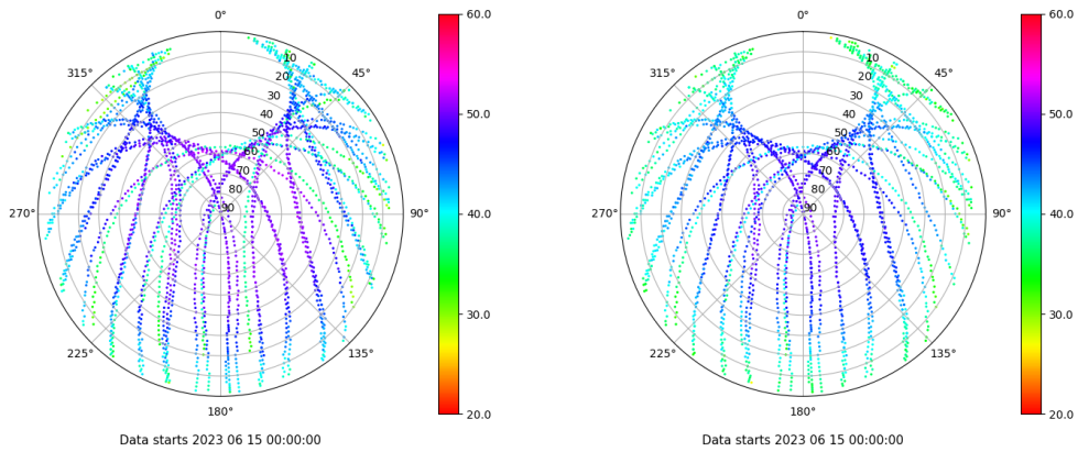
Skyplot for station BUIT. Signal to Noise S1C Data file BUIT00ESP_R_2023166.xtr Skyplot for station BUIT. Signal to Noise S2C Data file BUIT00ESP_R_2023166.xtr
