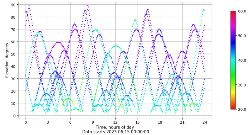
Time-elevation plot for station BUIT. Signal to Noise S1C Data file BUIT00ESP_R_2023166.xtr
