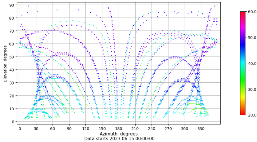
Azimuth-elevation plot for station BUIT. Signal to Noise S1C Data file BUIT00ESP_R_2023166.xtr
