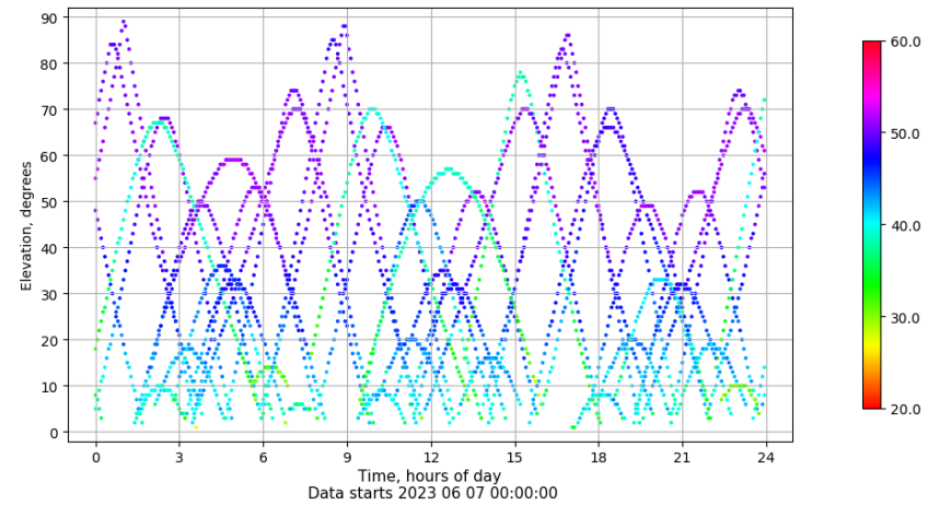
Time-elevation plot for station BUIT. Signal to Noise S1C Data file BUIT00ESP_R_2023158.xtr
