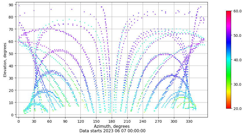
Azimuth-elevation plot for station BUIT. Signal to Noise S1C Data file BUIT00ESP_R_2023158.xtr
