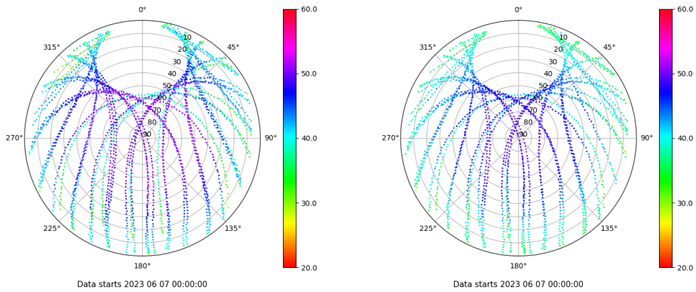
Skyplot for station BUIT. Signal to Noise S1C Data file BUIT00ESP_R_2023158.xtr Skyplot for station BUIT. Signal to Noise S2C Data file BUIT00ESP_R_2023158.xtr
