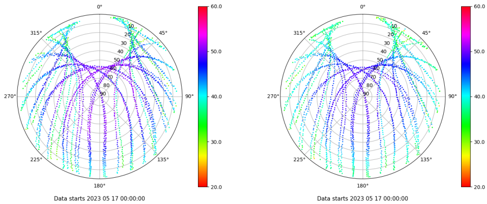
Skyplot for station BUIT. Signal to Noise S1C Data file BUIT00ESP_R_2023137.xtr Skyplot for station BUIT. Signal to Noise S2C Data file BUIT00ESP_R_2023137.xtr
