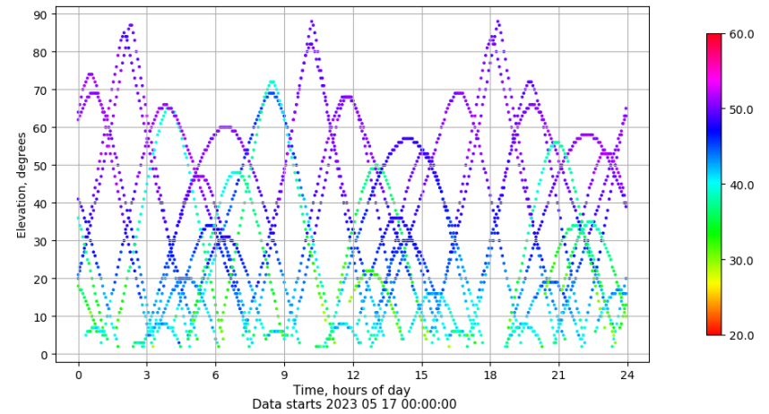
Time-elevation plot for station BUIT. Signal to Noise S1C Data file BUIT00ESP_R_2023137.xtr
