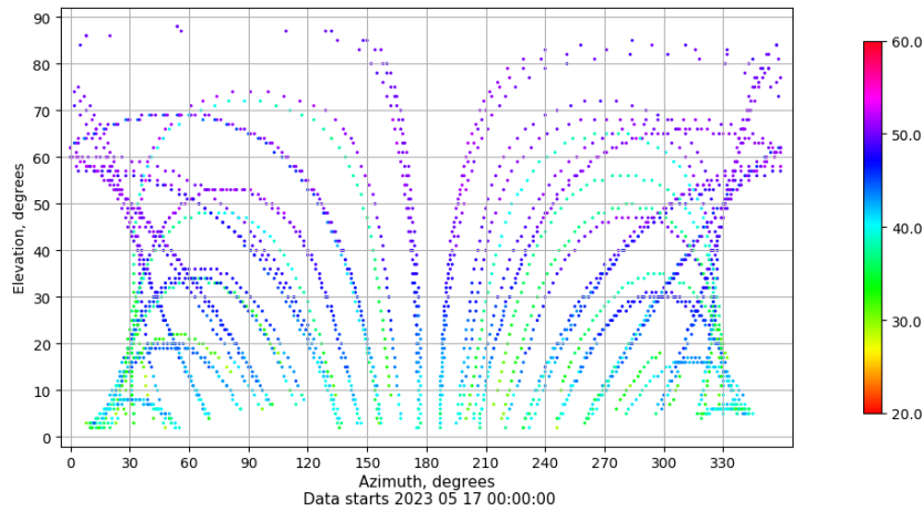
Azimuth-elevation plot for station BUIT. Signal to Noise S1C Data file BUIT00ESP_R_2023137.xtr
