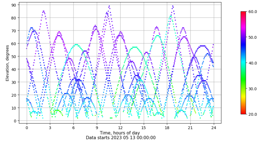
Time-elevation plot for station BUIT. Signal to Noise S1C Data file BUIT00ESP_R_2023133.xtr
