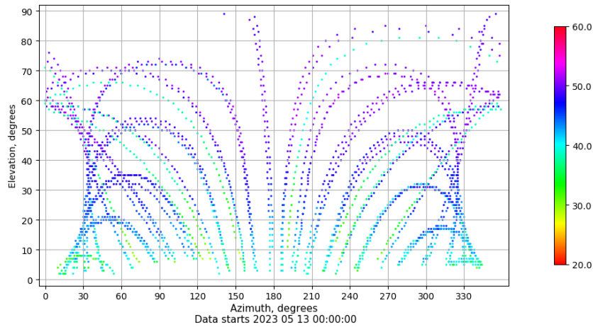
Azimuth-elevation plot for station BUIT. Signal to Noise S1C Data file BUIT00ESP_R_2023133.xtr
