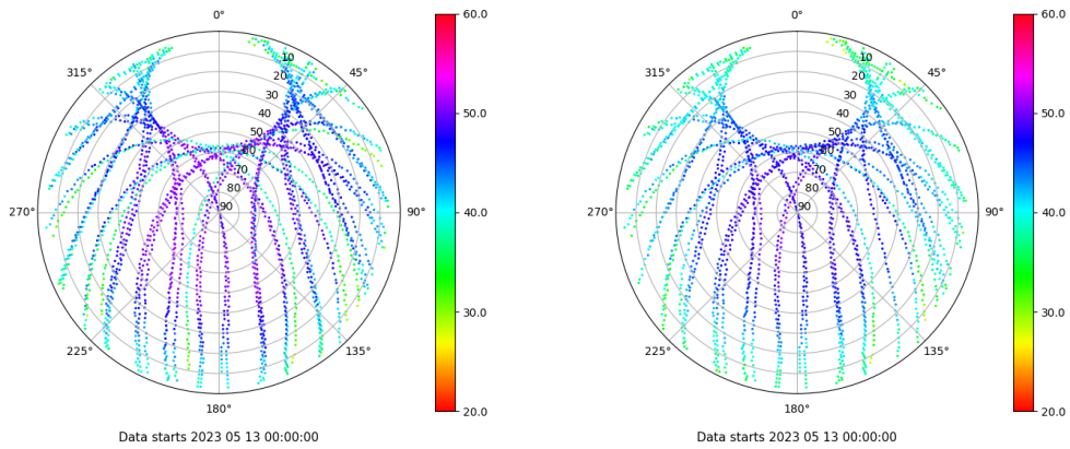
Skyplot for station BUIT. Signal to Noise S1C Data file BUIT00ESP_R_2023133.xtr Skyplot for station BUIT. Signal to Noise S2C Data file BUIT00ESP_R_2023133.xtr
