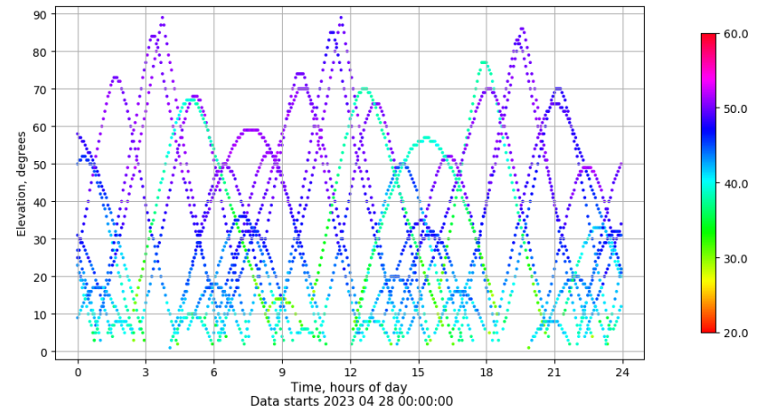
Time-elevation plot for station BUIT. Signal to Noise S1C Data file BUIT00ESP_R_2023118.xtr
