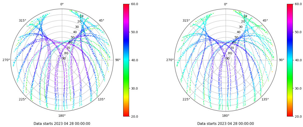
Skyplot for station BUIT. Signal to Noise S1C Data file BUIT00ESP_R_2023118.xtr Skyplot for station BUIT. Signal to Noise S2C Data file BUIT00ESP_R_2023118.xtr
