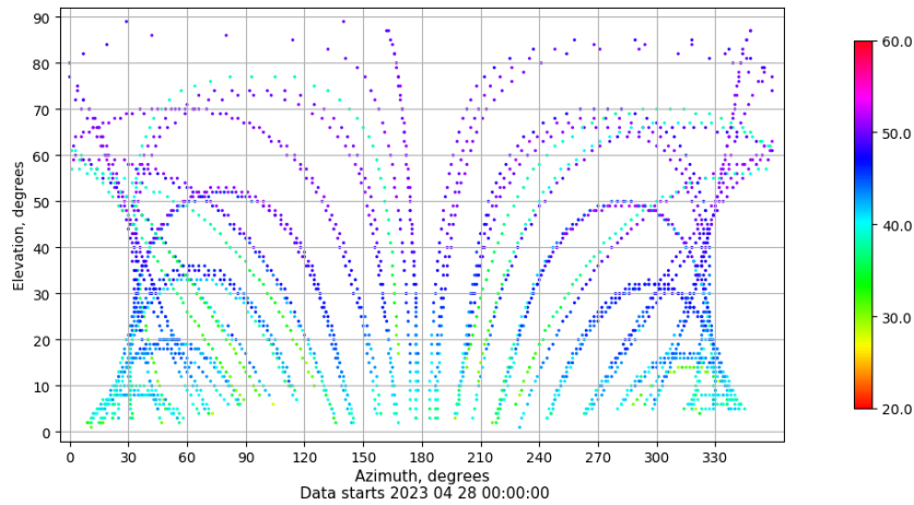
Azimuth-elevation plot for station BUIT. Signal to Noise S1C Data file BUIT00ESP_R_2023118.xtr
