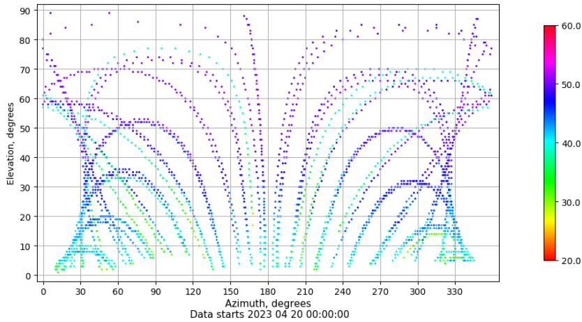
Azimuth-elevation plot for station BUIT. Signal to Noise S1C Data file BUIT00ESP_R_2023110.xtr
