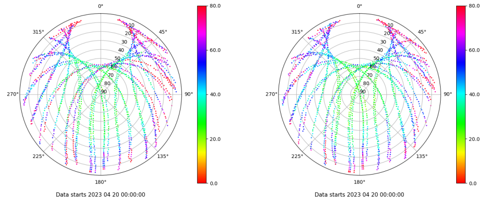
Skyplot for station BUIT. Parameter M1C Data file BUIT00ESP_R_2023110.xtr Skyplot for station BUIT. Parameter M2C Data file BUIT00ESP_R_2023110.xtr
