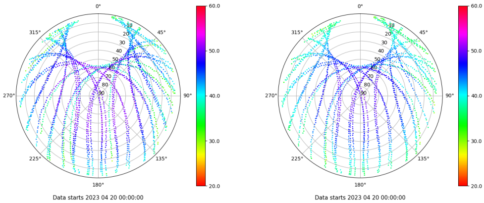
Skyplot for station BUIT. Signal to Noise S1C Data file BUIT00ESP_R_2023110.xtr Skyplot for station BUIT. Signal to Noise S2C Data file BUIT00ESP_R_2023110.xtr
