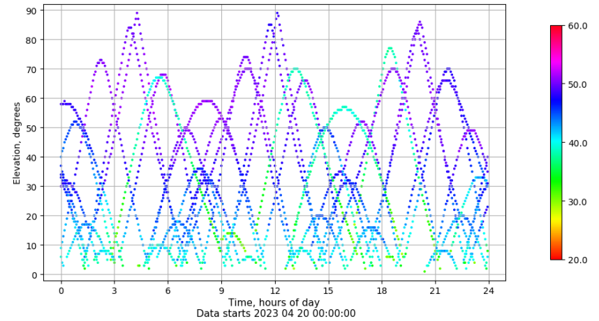
Time-elevation plot for station BUIT. Signal to Noise S1C Data file BUIT00ESP_R_2023110.xtr
