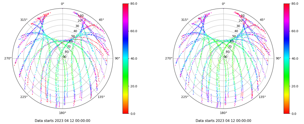
Skyplot for station BUIT. Parameter M1C Data file BUIT00ESP_R_2023102.xtr Skyplot for station BUIT. Parameter M2C Data file BUIT00ESP_R_2023102.xtr
