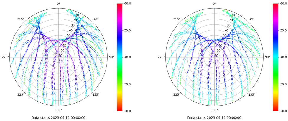
Skyplot for station BUIT. Signal to Noise S1C Data file BUIT00ESP_R_2023102.xtr Skyplot for station BUIT. Signal to Noise S2C Data file BUIT00ESP_R_2023102.xtr
