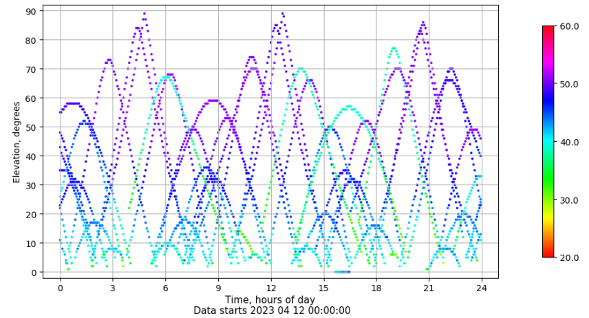
Time-elevation plot for station BUIT. Signal to Noise S1C Data file BUIT00ESP_R_2023102.xtr
