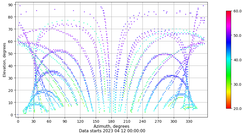
Azimuth-elevation plot for station BUIT. Signal to Noise S1C Data file BUIT00ESP_R_2023102.xtr
