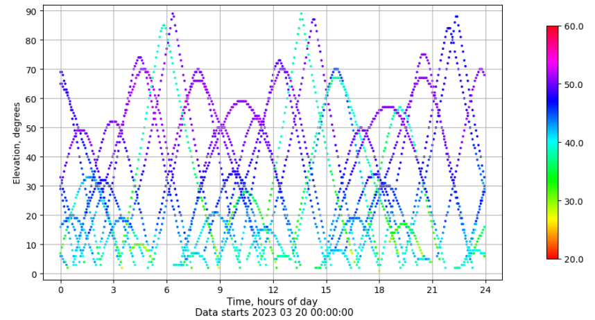
Time-elevation plot for station BUIT. Signal to Noise S1C Data file BUIT00ESP_R_2023079.xtr
