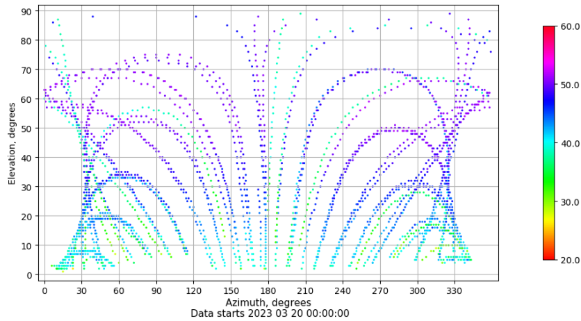
Azimuth-elevation plot for station BUIT. Signal to Noise S1C Data file BUIT00ESP_R_2023079.xtr
