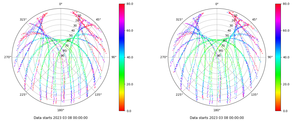
Skyplot for station BUIT. Parameter M1C Data file BUIT00ESP_R_2023067.xtr Skyplot for station BUIT. Parameter M2C Data file BUIT00ESP_R_2023067.xtr
