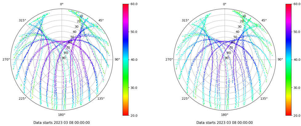
Skyplot for station BUIT. Signal to Noise S1C Data file BUIT00ESP_R_2023067.xtr Skyplot for station BUIT. Signal to Noise S2C Data file BUIT00ESP_R_2023067.xtr
