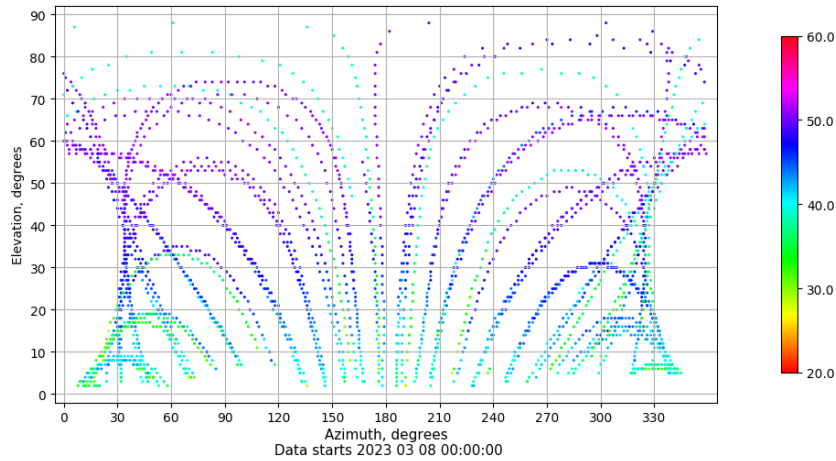
Azimuth-elevation plot for station BUIT. Signal to Noise S1C Data file BUIT00ESP_R_2023067.xtr
