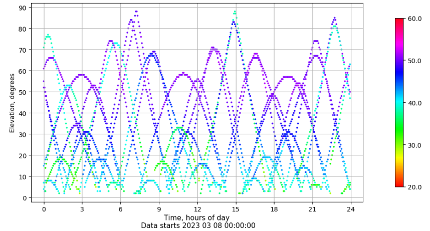
Time-elevation plot for station BUIT. Signal to Noise S1C Data file BUIT00ESP_R_2023067.xtr
