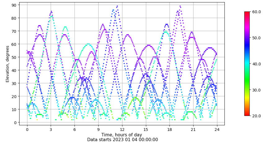
Time-elevation plot for station BUIT. Signal to Noise S1C Data file BUIT00ESP_R_2023004.xtr
