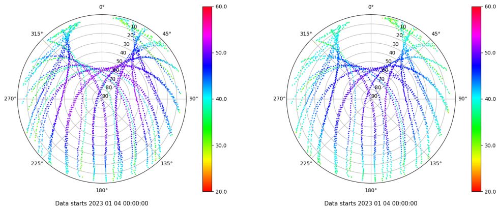
Skyplot for station BUIT. Signal to Noise S1C Data file BUIT00ESP_R_2023004.xtr Skyplot for station BUIT. Signal to Noise S2C Data file BUIT00ESP_R_2023004.xtr
