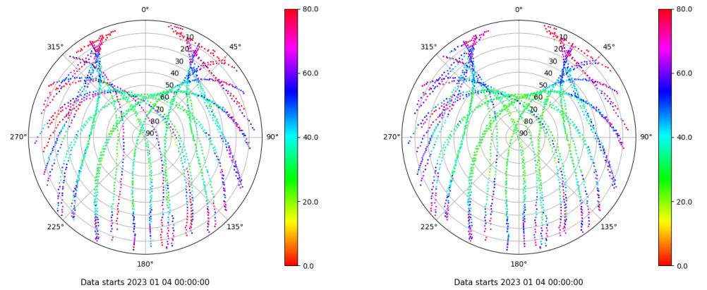
Skyplot for station BUIT. Parameter M1C Data file BUIT00ESP_R_2023004.xtr Skyplot for station BUIT. Parameter M2C Data file BUIT00ESP_R_2023004.xtr
