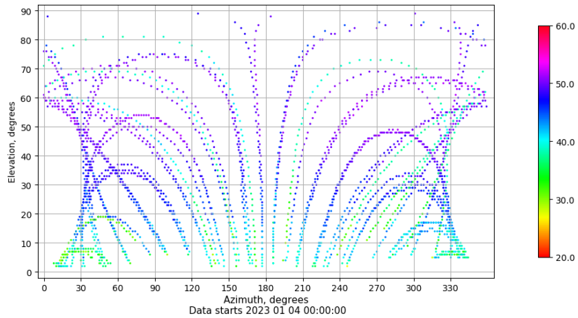
Azimuth-elevation plot for station BUIT. Signal to Noise S1C Data file BUIT00ESP_R_2023004.xtr
