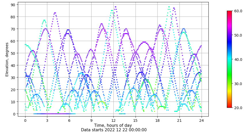
Time-elevation plot for station BUIT. Signal to Noise S1C Data file BUIT00ESP_R_2022356.xtr
