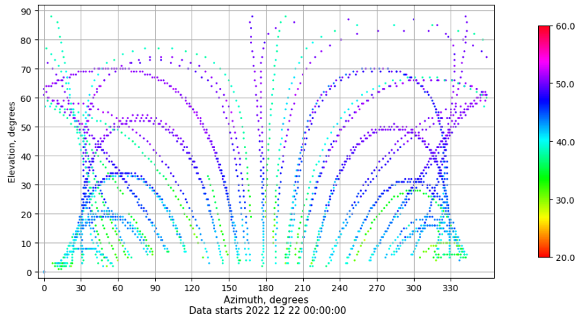
Azimuth-elevation plot for station BUIT. Signal to Noise S1C Data file BUIT00ESP_R_2022356.xtr
