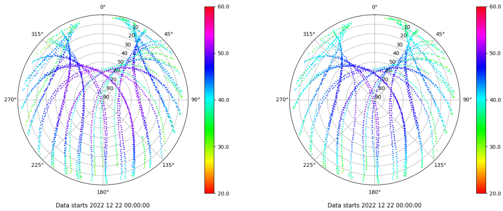
Skyplot for station BUIT. Signal to Noise S1C Data file BUIT00ESP_R_2022356.xtr Skyplot for station BUIT. Signal to Noise S2C Data file BUIT00ESP_R_2022356.xtr
