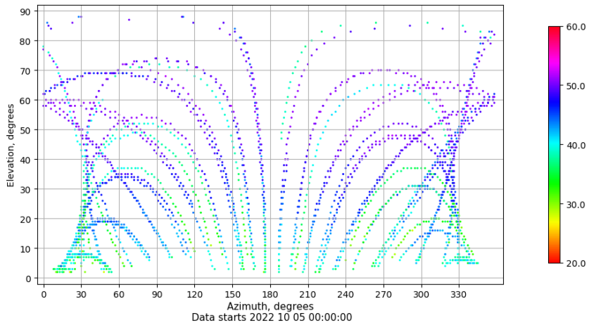
Azimuth-elevation plot for station BUIT. Signal to Noise S1C Data file BUIT00ESP_R_2022278.xtr
