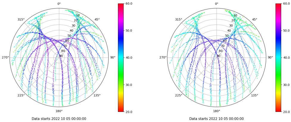
Skyplot for station BUIT. Signal to Noise S1C Data file BUIT00ESP_R_2022278.xtr Skyplot for station BUIT. Signal to Noise S2C Data file BUIT00ESP_R_2022278.xtr
