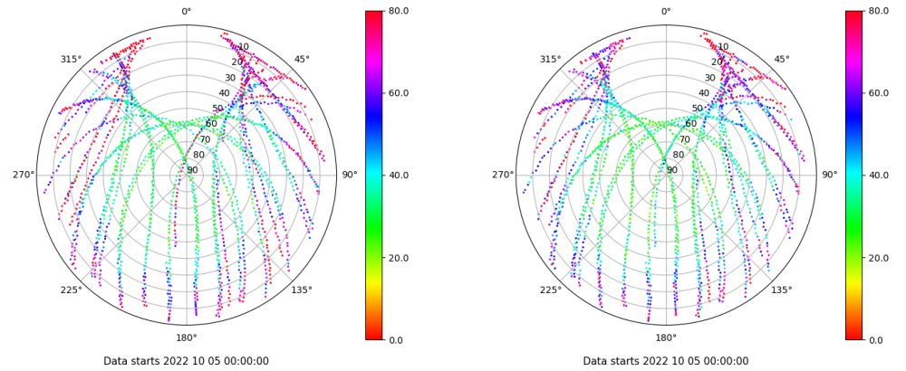
Skyplot for station BUIT. Parameter M1C Data file BUIT00ESP_R_2022278.xtr Skyplot for station BUIT. Parameter M2C Data file BUIT00ESP_R_2022278.xtr
