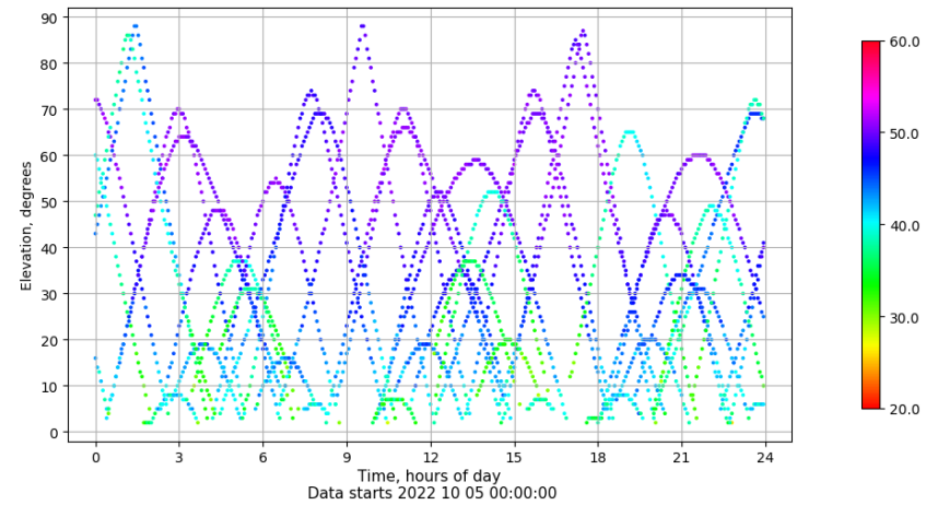
Time-elevation plot for station BUIT. Signal to Noise S1C Data file BUIT00ESP_R_2022278.xtr
