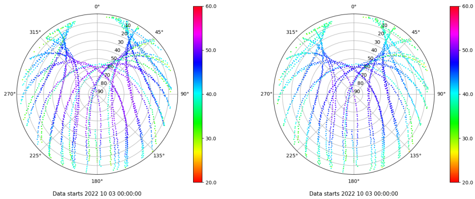
Skyplot for station BUIT. Signal to Noise S1C Data file BUIT00ESP_R_2022276.xtr Skyplot for station BUIT. Signal to Noise S2C Data file BUIT00ESP_R_2022276.xtr
