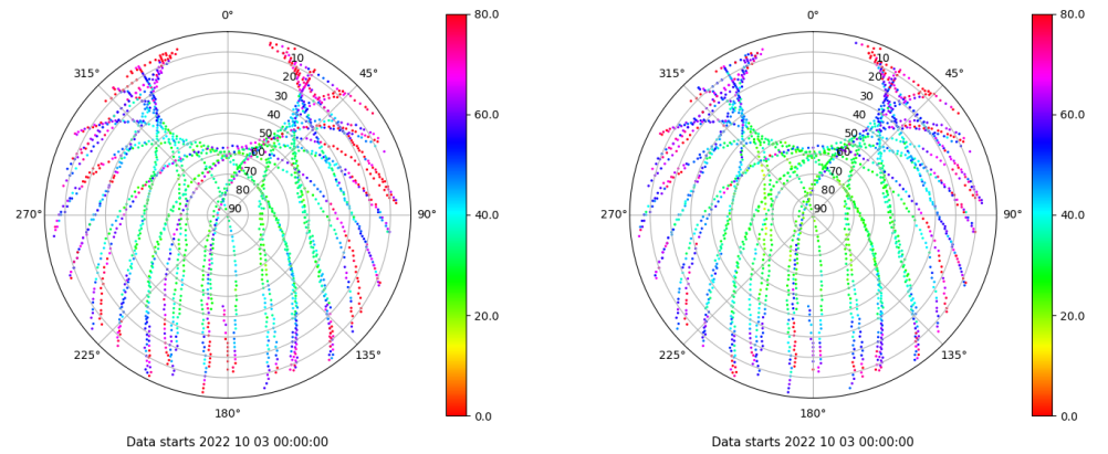
Skyplot for station BUIT. Parameter M1C Data file BUIT00ESP_R_2022276.xtr Skyplot for station BUIT. Parameter M2C Data file BUIT00ESP_R_2022276.xtr
