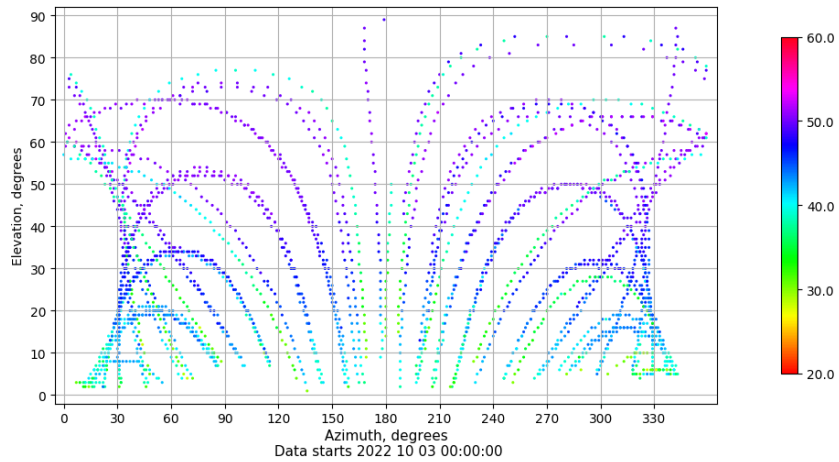
Azimuth-elevation plot for station BUIT. Signal to Noise S1C Data file BUIT00ESP_R_2022276.xtr
