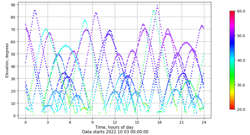
Time-elevation plot for station BUIT. Signal to Noise S1C Data file BUIT00ESP_R_2022276.xtr
