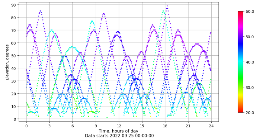
Time-elevation plot for station BUIT. Signal to Noise S1C Data file BUIT00ESP_R_2022268.xtr
