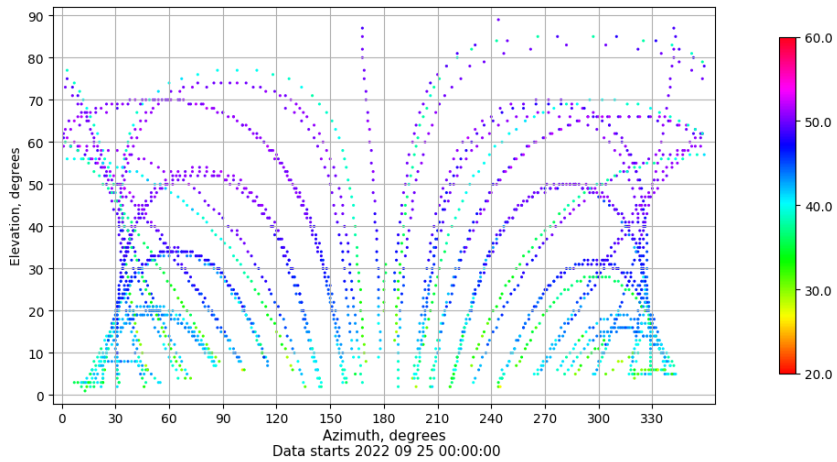
Azimuth-elevation plot for station BUIT. Signal to Noise S1C Data file BUIT00ESP_R_2022268.xtr
