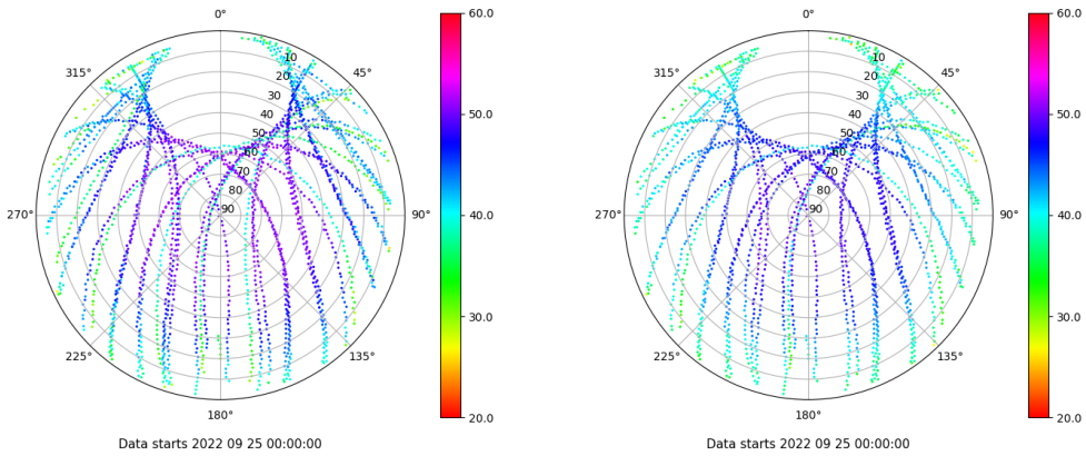
Skyplot for station BUIT. Signal to Noise S1C Data file BUIT00ESP_R_2022268.xtr Skyplot for station BUIT. Signal to Noise S2C Data file BUIT00ESP_R_2022268.xtr
