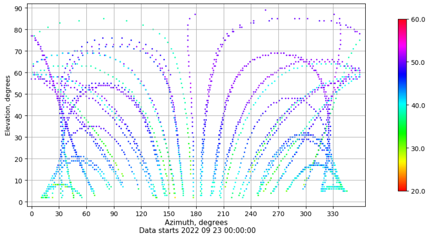
Azimuth-elevation plot for station BUIT. Signal to Noise S1C Data file BUIT00ESP_R_2022266.xtr
