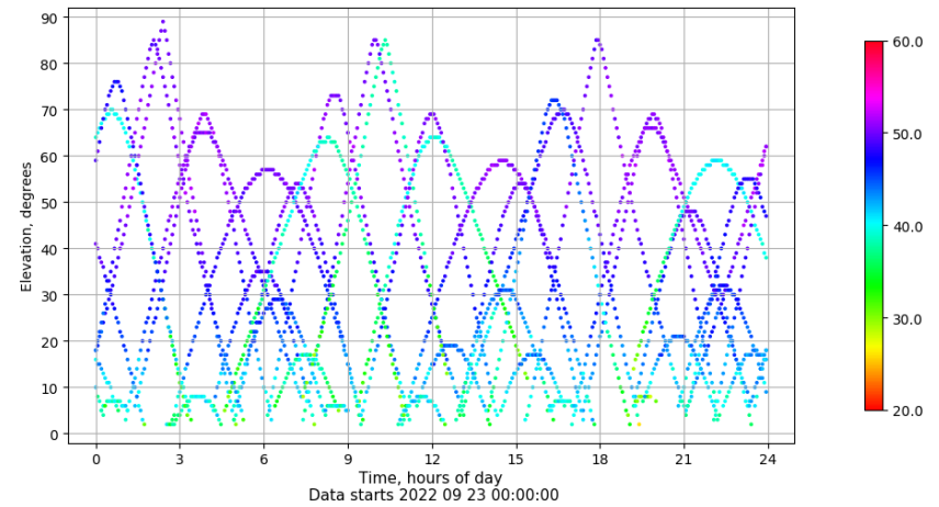
Time-elevation plot for station BUIT. Signal to Noise S1C Data file BUIT00ESP_R_2022266.xtr
