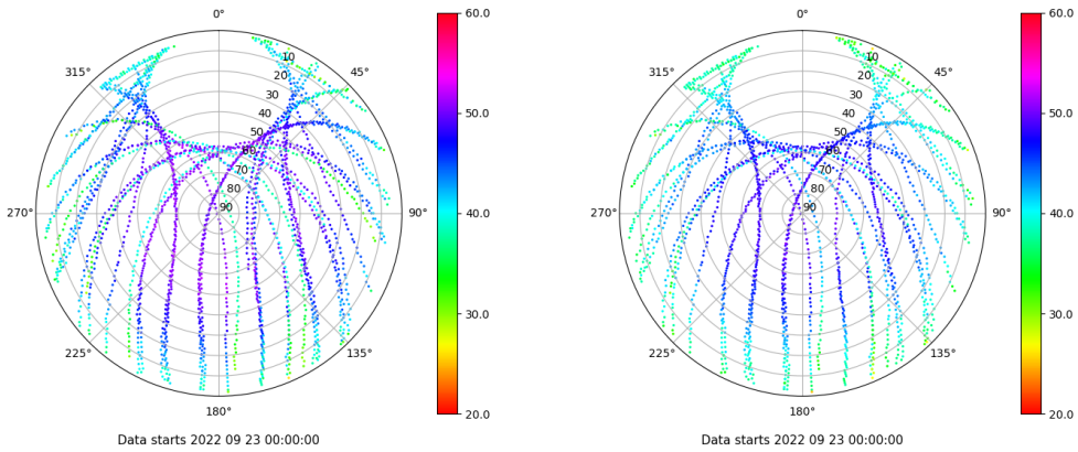
Skyplot for station BUIT. Signal to Noise S1C Data file BUIT00ESP_R_2022266.xtr Skyplot for station BUIT. Signal to Noise S2C Data file BUIT00ESP_R_2022266.xtr
