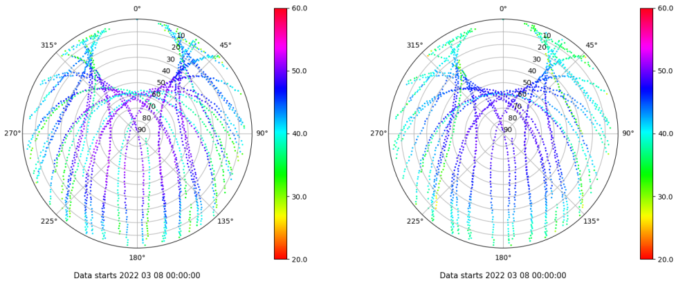
Skyplot for station BUIT. Signal to Noise S1C Data file BUIT00ESP_R_2022067.xtr Skyplot for station BUIT. Signal to Noise S2C Data file BUIT00ESP_R_2022067.xtr
