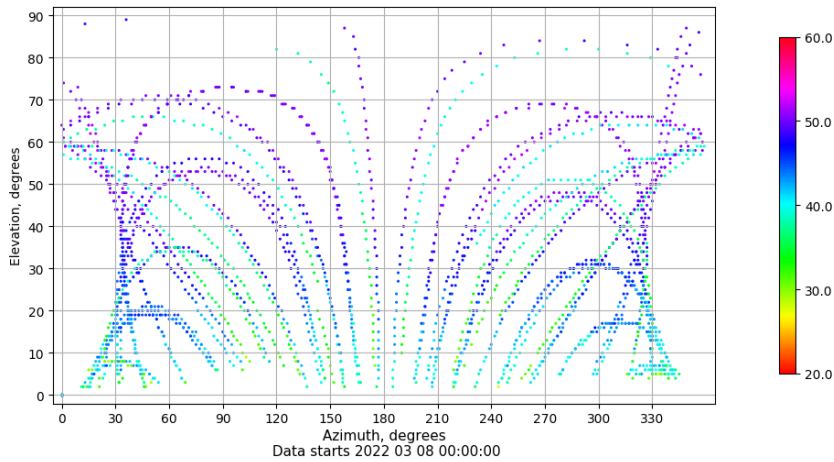
Azimuth-elevation plot for station BUIT. Signal to Noise S1C Data file BUIT00ESP_R_2022067.xtr
