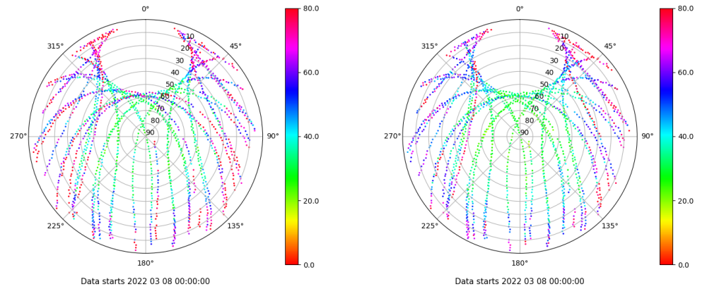
Skyplot for station BUIT. Parameter M1C Data file BUIT00ESP_R_2022067.xtr Skyplot for station BUIT. Parameter M2C Data file BUIT00ESP_R_2022067.xtr
