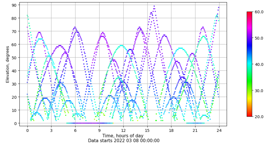
Time-elevation plot for station BUIT. Signal to Noise S1C Data file BUIT00ESP_R_2022067.xtr
