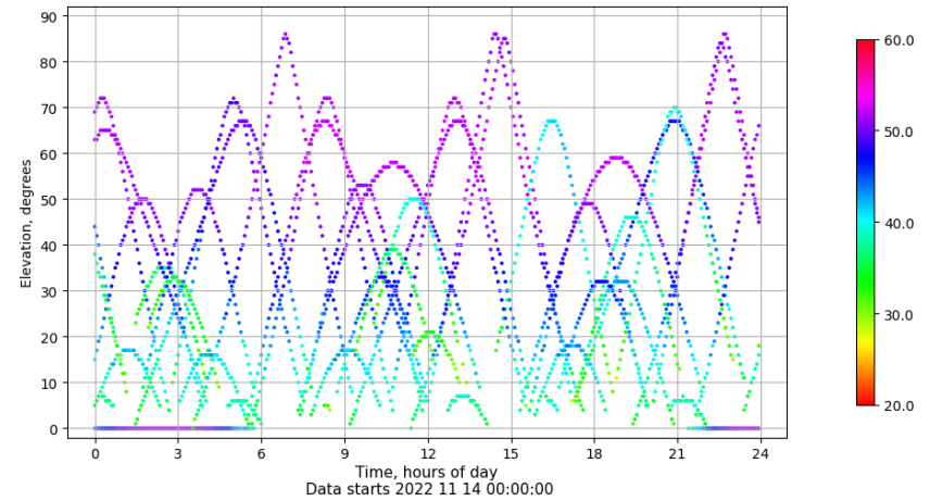
Time-elevation plot for station BEJR. Signal to Noise S1C Data file BEJR00ESP_R_2022318.xtr
