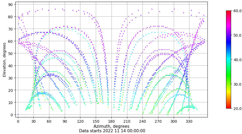
Azimuth-elevation plot for station BEJR. Signal to Noise S1C Data file BEJR00ESP_R_2022318.xtr
