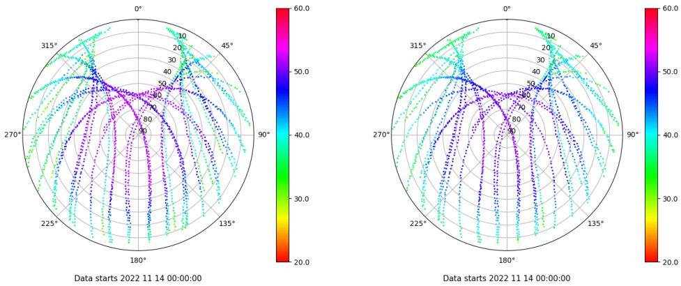
Skyplot for station BEJR. Signal to Noise S1C Data file BEJR00ESP_R_2022318.xtr Skyplot for station BEJR. Signal to Noise S2C Data file BEJR00ESP_R_2022318.xtr
