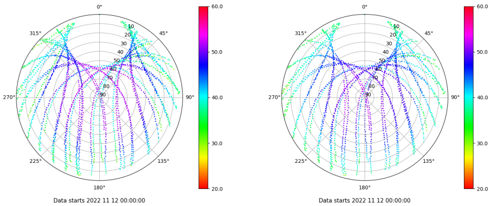
Skyplot for station BEJR. Signal to Noise S1C Data file BEJR00ESP_R_2022316.xtr Skyplot for station BEJR. Signal to Noise S2C Data file BEJR00ESP_R_2022316.xtr
