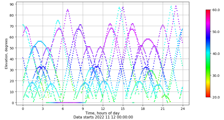
Time-elevation plot for station BEJR. Signal to Noise S1C Data file BEJR00ESP_R_2022316.xtr
