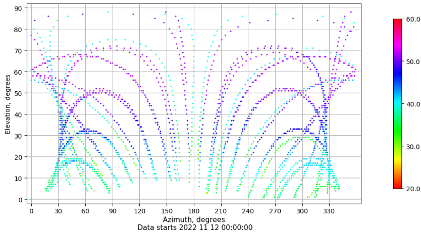
Azimuth-elevation plot for station BEJR. Signal to Noise S1C Data file BEJR00ESP_R_2022316.xtr
