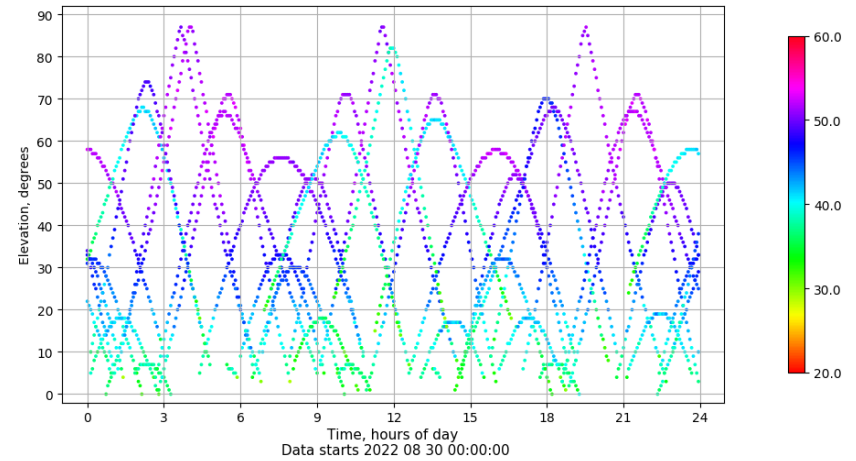
Time-elevation plot for station BEJR. Signal to Noise S1C Data file BEJR00ESP_R_2022242.xtr
