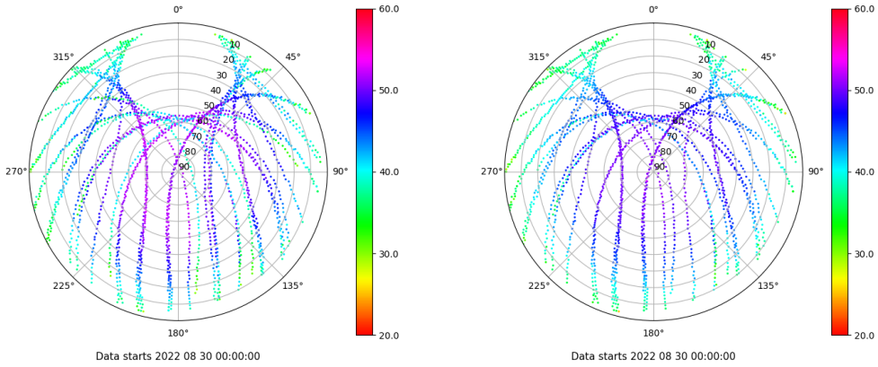
Skyplot for station BEJR. Signal to Noise S1C Data file BEJR00ESP_R_2022242.xtr Skyplot for station BEJR. Signal to Noise S2C Data file BEJR00ESP_R_2022242.xtr
