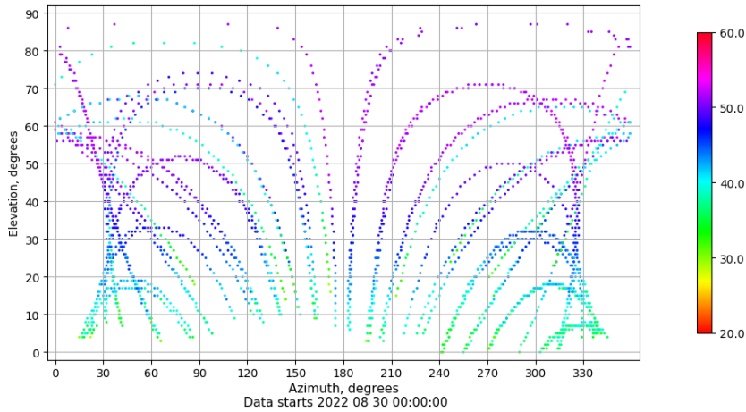
Azimuth-elevation plot for station BEJR. Signal to Noise S1C Data file BEJR00ESP_R_2022242.xtr
