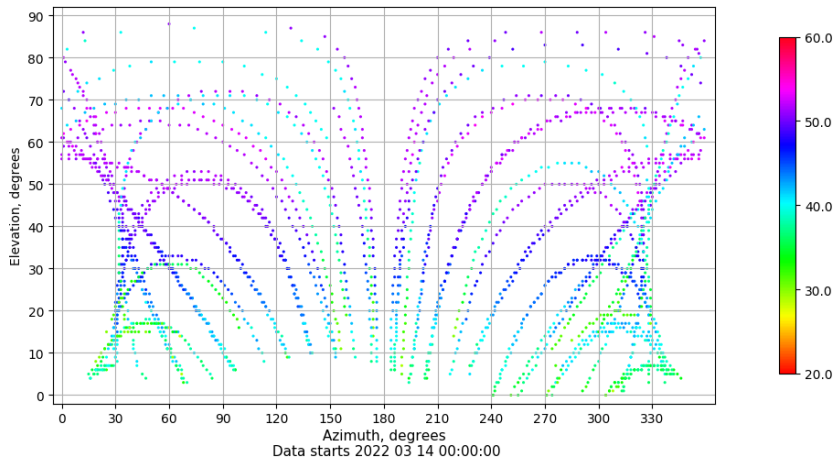
Azimuth-elevation plot for station BEJR. Signal to Noise S1C Data file BEJR00ESP_R_2022073.xtr
