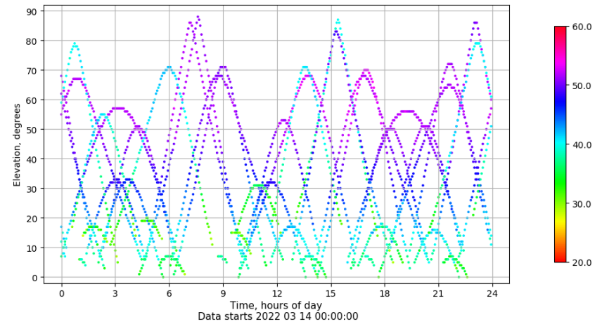
Time-elevation plot for station BEJR. Signal to Noise S1C Data file BEJR00ESP_R_2022073.xtr
