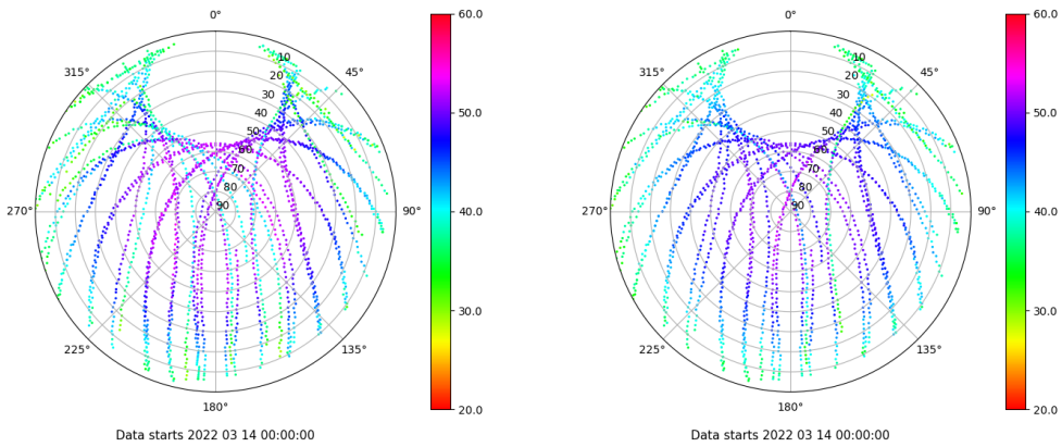
Skyplot for station BEJR. Signal to Noise S1C Data file BEJR00ESP_R_2022073.xtr Skyplot for station BEJR. Signal to Noise S2C Data file BEJR00ESP_R_2022073.xtr
