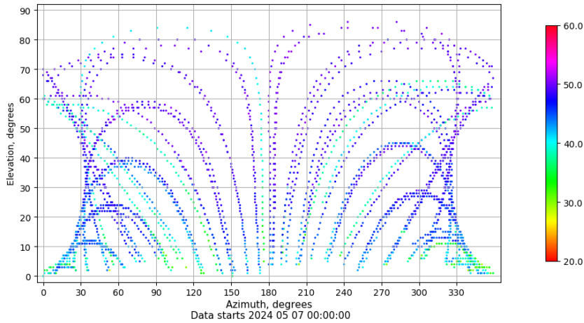
Azimuth-elevation plot for station BCLN. Signal to Noise S1C Data file BCLN00ESP_R_2024128.xtr
