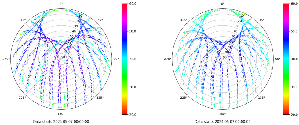
Skyplot for station BCLN. Signal to Noise S1C Data file BCLN00ESP_R_2024128.xtr Skyplot for station BCLN. Signal to Noise S2P Data file BCLN00ESP_R_2024128.xtr
