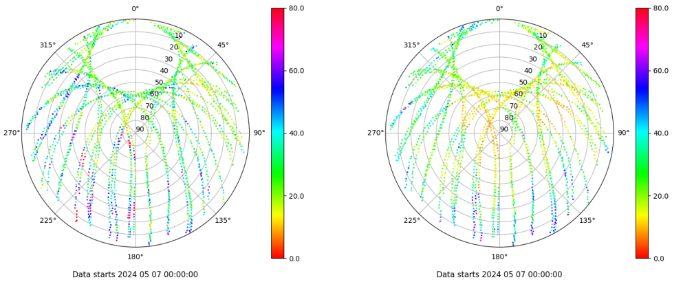
Skyplot for station BCLN. Parameter M1C Data file BCLN00ESP_R_2024128.xtr Skyplot for station BCLN. Parameter M2P Data file BCLN00ESP_R_2024128.xtr
