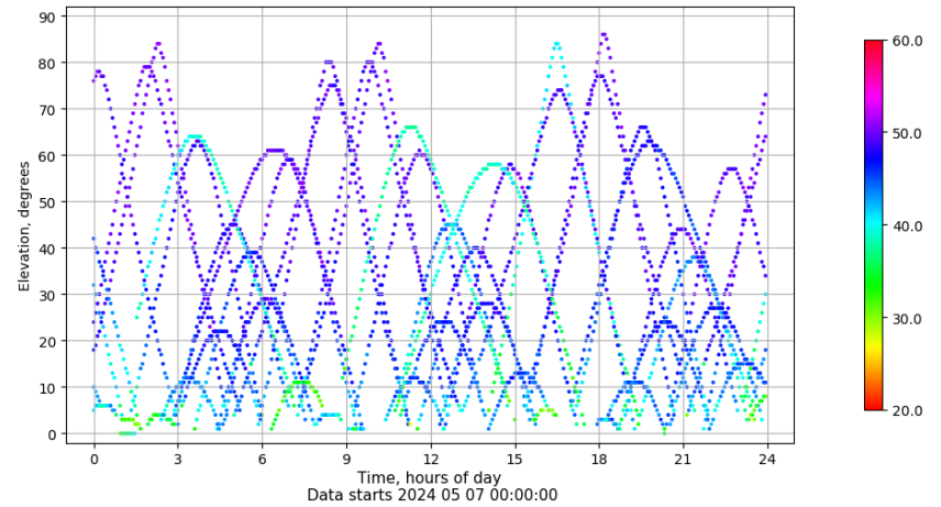
Time-elevation plot for station BCLN. Signal to Noise S1C Data file BCLN00ESP_R_2024128.xtr
