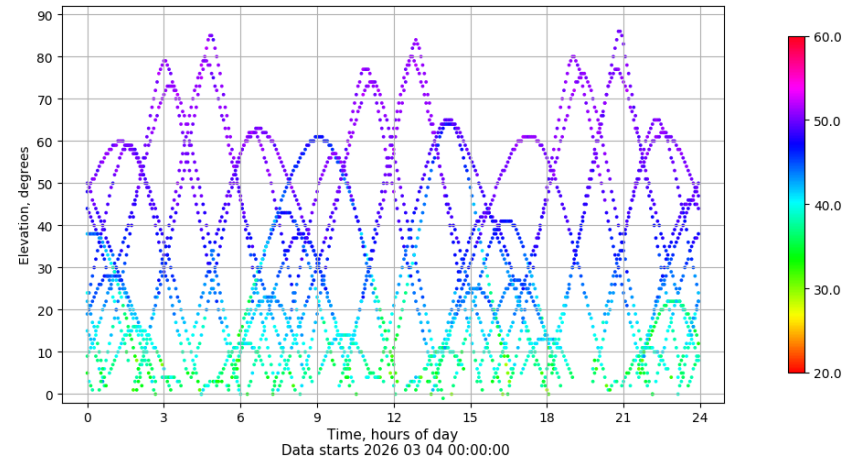
Time-elevation plot for station BCL1. Signal to Noise S1C Data file BCL100ESP_R_2026063.xtr
