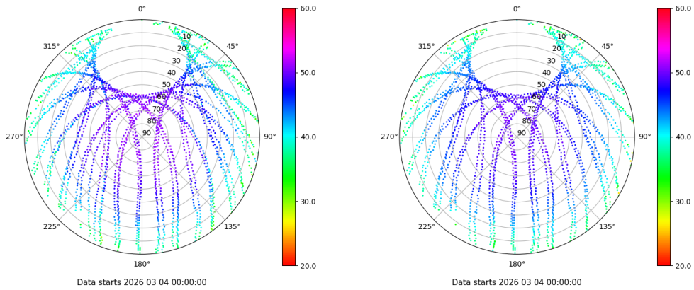
Skyplot for station BCL1. Signal to Noise S1C Data file BCL100ESP_R_2026063.xtr Skyplot for station BCL1. Signal to Noise S2P Data file BCL100ESP_R_2026063.xtr
