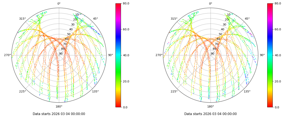
Skyplot for station BCL1. Parameter M1C Data file BCL100ESP_R_2026063.xtr Skyplot for station BCL1. Parameter M2P Data file BCL100ESP_R_2026063.xtr
