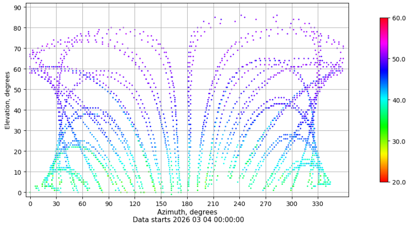
Azimuth-elevation plot for station BCL1. Signal to Noise S1C Data file BCL100ESP_R_2026063.xtr
