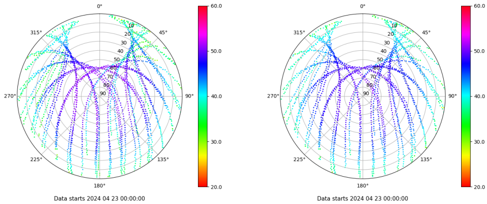
Skyplot for station BCL1. Signal to Noise S1C Data file BCL100ESP_R_2024114.xtr Skyplot for station BCL1. Signal to Noise S2P Data file BCL100ESP_R_2024114.xtr
