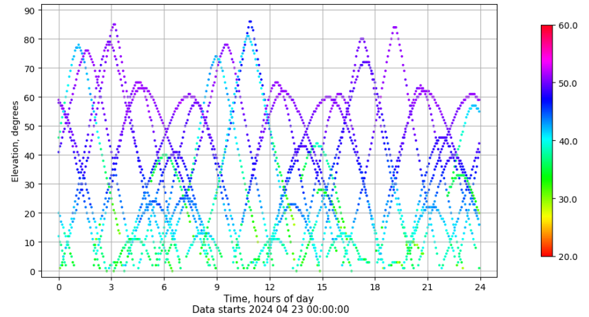
Time-elevation plot for station BCL1. Signal to Noise S1C Data file BCL100ESP_R_2024114.xtr
