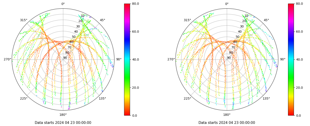
Skyplot for station BCL1. Parameter M1C Data file BCL100ESP_R_2024114.xtr Skyplot for station BCL1. Parameter M2P Data file BCL100ESP_R_2024114.xtr
