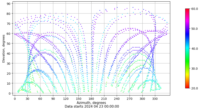
Azimuth-elevation plot for station BCL1. Signal to Noise S1C Data file BCL100ESP_R_2024114.xtr
