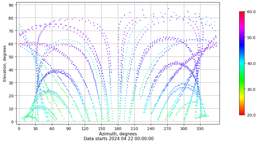
Azimuth-elevation plot for station BCL1. Signal to Noise S1C Data file BCL100ESP_R_2024113.xtr
