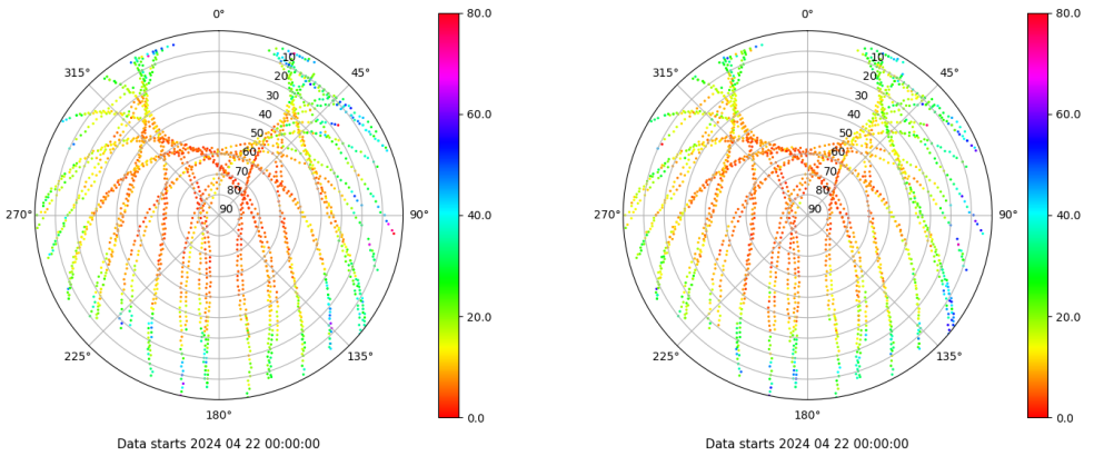
Skyplot for station BCL1. Parameter M1C Data file BCL100ESP_R_2024113.xtr Skyplot for station BCL1. Parameter M2P Data file BCL100ESP_R_2024113.xtr
