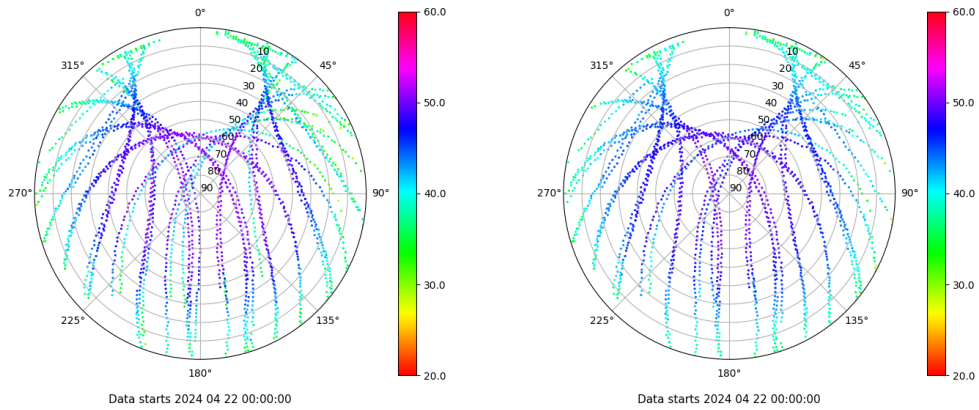
Skyplot for station BCL1. Signal to Noise S1C Data file BCL100ESP_R_2024113.xtr Skyplot for station BCL1. Signal to Noise S2P Data file BCL100ESP_R_2024113.xtr
