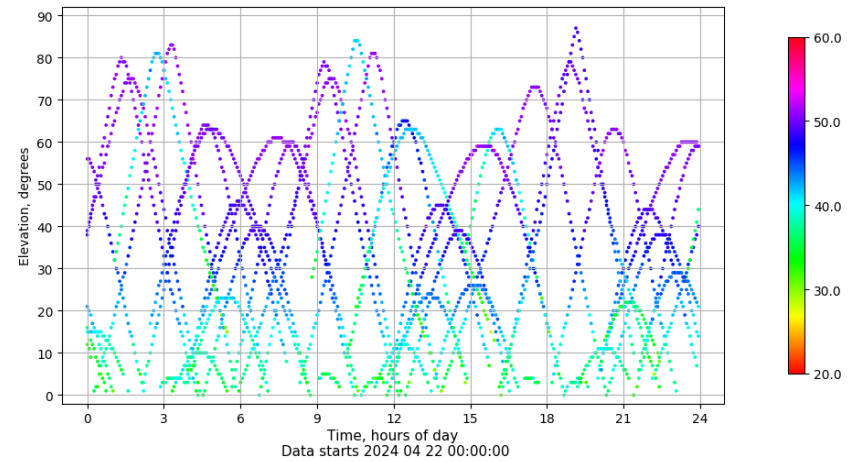
Time-elevation plot for station BCL1. Signal to Noise S1C Data file BCL100ESP_R_2024113.xtr
