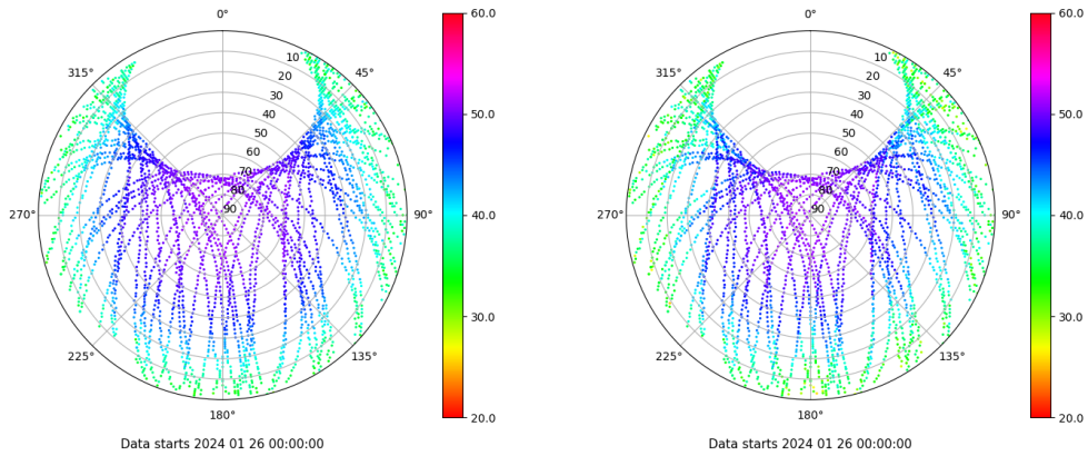
Skyplot for station BCL1. Signal to Noise S1C Data file BCL100ESP_R_2024026.xtr Skyplot for station BCL1. Signal to Noise S2W Data file BCL100ESP_R_2024026.xtr
