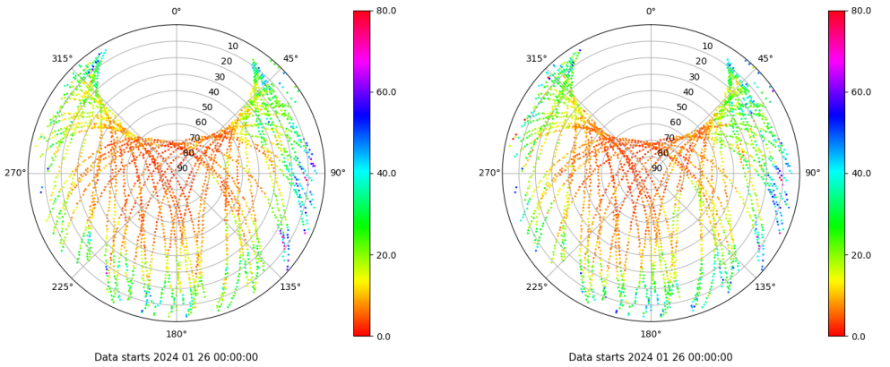
Skyplot for station BCL1. Parameter M1C Data file BCL100ESP_R_2024026.xtr Skyplot for station BCL1. Parameter M2W Data file BCL100ESP_R_2024026.xtr
