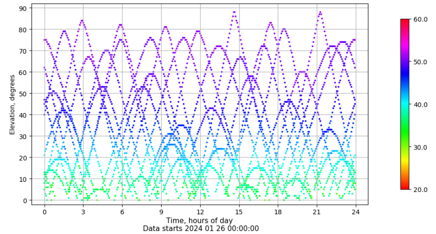
Time-elevation plot for station BCL1. Signal to Noise S1C Data file BCL100ESP_R_2024026.xtr
