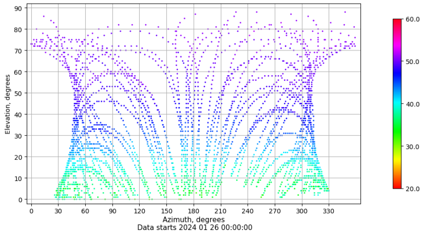
Azimuth-elevation plot for station BCL1. Signal to Noise S1C Data file BCL100ESP_R_2024026.xtr
