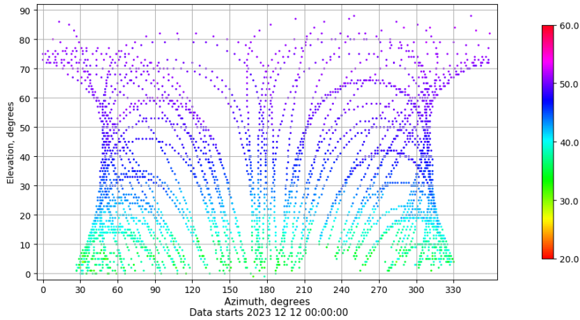
Azimuth-elevation plot for station BCL1. Signal to Noise S1C Data file BCL100ESP_R_2023346.xtr
