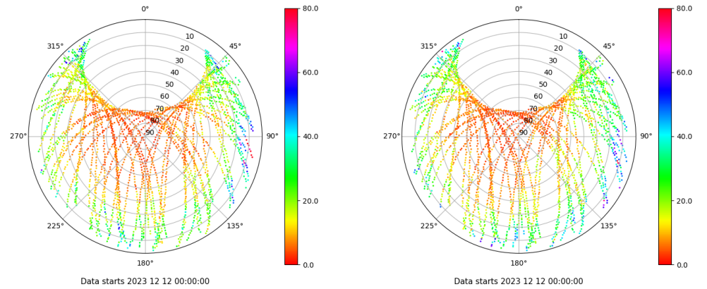
Skyplot for station BCL1. Parameter M1C Data file BCL100ESP_R_2023346.xtr Skyplot for station BCL1. Parameter M2W Data file BCL100ESP_R_2023346.xtr
