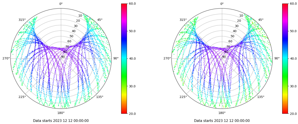
Skyplot for station BCL1. Signal to Noise S1C Data file BCL100ESP_R_2023346.xtr Skyplot for station BCL1. Signal to Noise S2W Data file BCL100ESP_R_2023346.xtr
