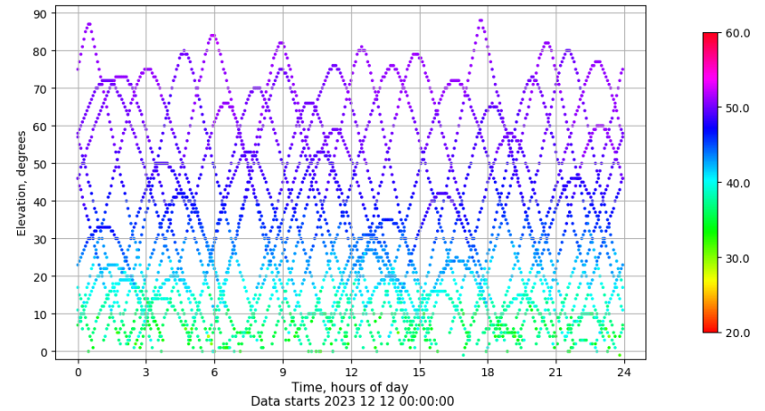
Time-elevation plot for station BCL1. Signal to Noise S1C Data file BCL100ESP_R_2023346.xtr
