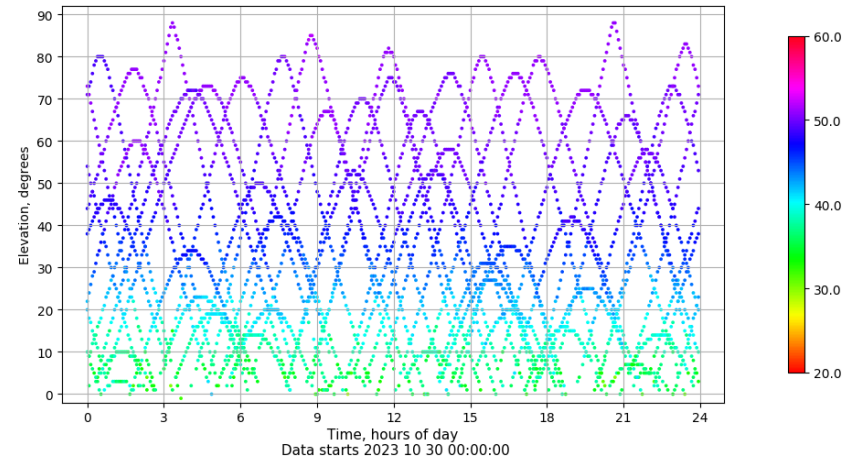
Time-elevation plot for station BCL1. Signal to Noise S1C Data file BCL100ESP_R_2023303.xtr
