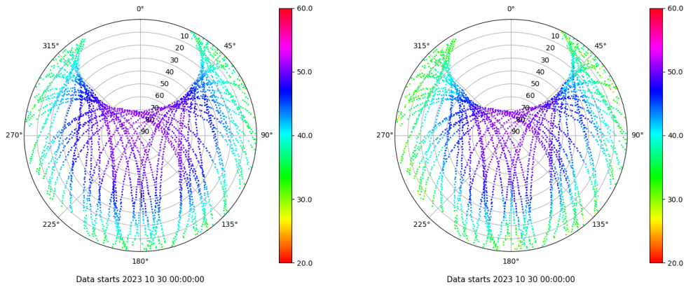
Skyplot for station BCL1. Signal to Noise S1C Data file BCL100ESP_R_2023303.xtr Skyplot for station BCL1. Signal to Noise S2W Data file BCL100ESP_R_2023303.xtr
