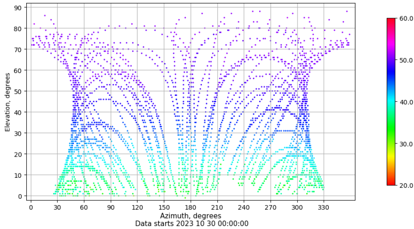
Azimuth-elevation plot for station BCL1. Signal to Noise S1C Data file BCL100ESP_R_2023303.xtr
