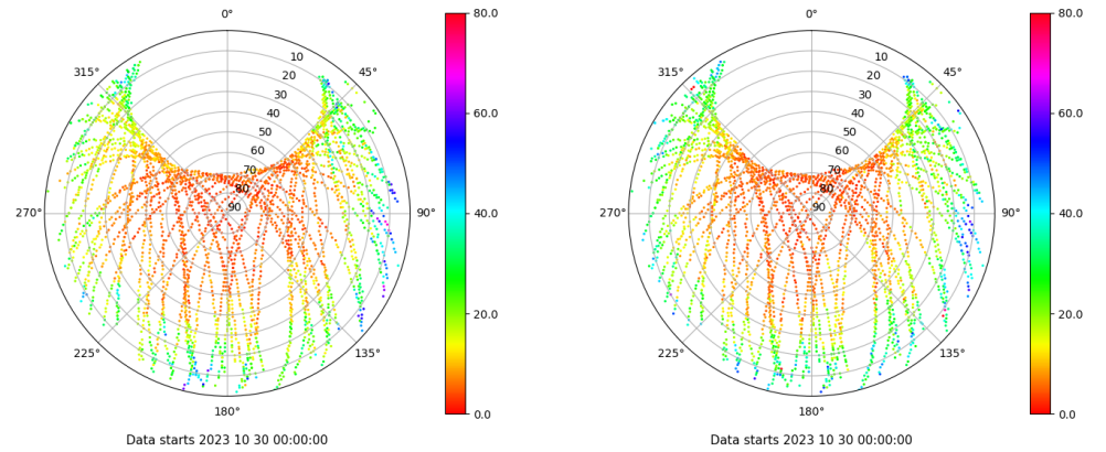
Skyplot for station BCL1. Parameter M1C Data file BCL100ESP_R_2023303.xtr Skyplot for station BCL1. Parameter M2W Data file BCL100ESP_R_2023303.xtr
