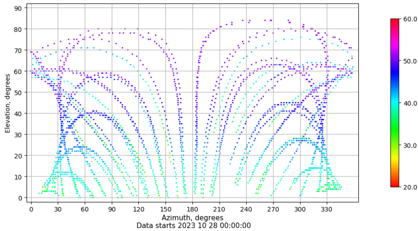
Azimuth-elevation plot for station BCL1. Signal to Noise S1C Data file BCL100ESP_R_2023301.xtr
