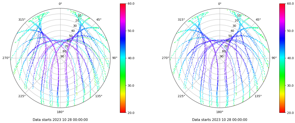
Skyplot for station BCL1. Signal to Noise S1C Data file BCL100ESP_R_2023301.xtr Skyplot for station BCL1. Signal to Noise S2P Data file BCL100ESP_R_2023301.xtr
