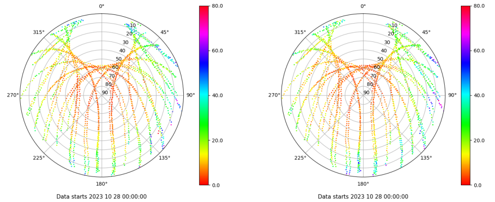
Skyplot for station BCL1. Parameter M1C Data file BCL100ESP_R_2023301.xtr Skyplot for station BCL1. Parameter M2P Data file BCL100ESP_R_2023301.xtr
