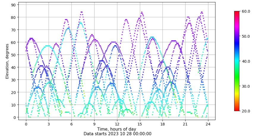
Time-elevation plot for station BCL1. Signal to Noise S1C Data file BCL100ESP_R_2023301.xtr
