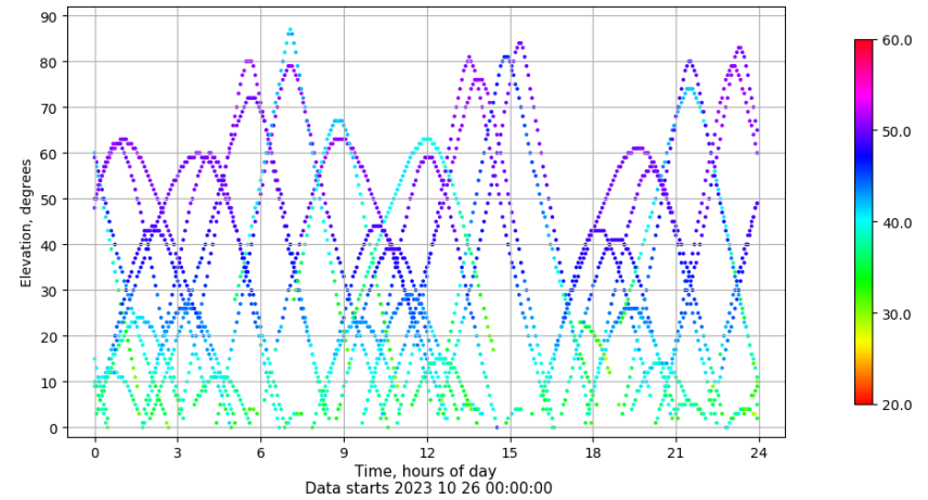
Time-elevation plot for station BCL1. Signal to Noise S1C Data file BCL100ESP_R_2023299.xtr
