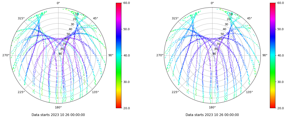
Skyplot for station BCL1. Signal to Noise S1C Data file BCL100ESP_R_2023299.xtr Skyplot for station BCL1. Signal to Noise S2P Data file BCL100ESP_R_2023299.xtr
