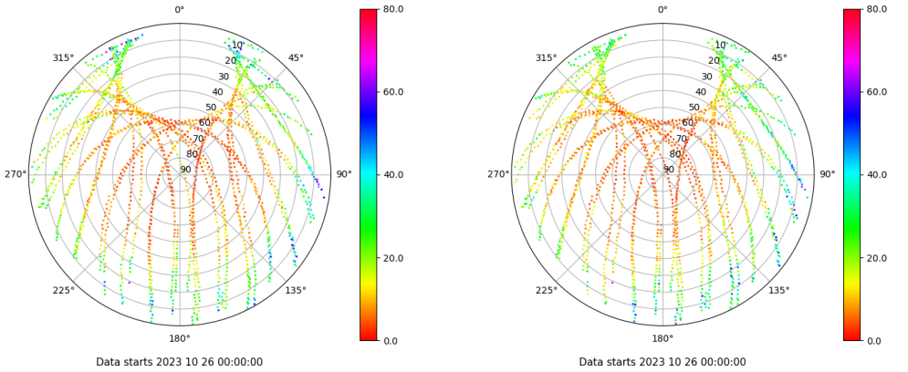
Skyplot for station BCL1. Parameter M1C Data file BCL100ESP_R_2023299.xtr Skyplot for station BCL1. Parameter M2P Data file BCL100ESP_R_2023299.xtr
