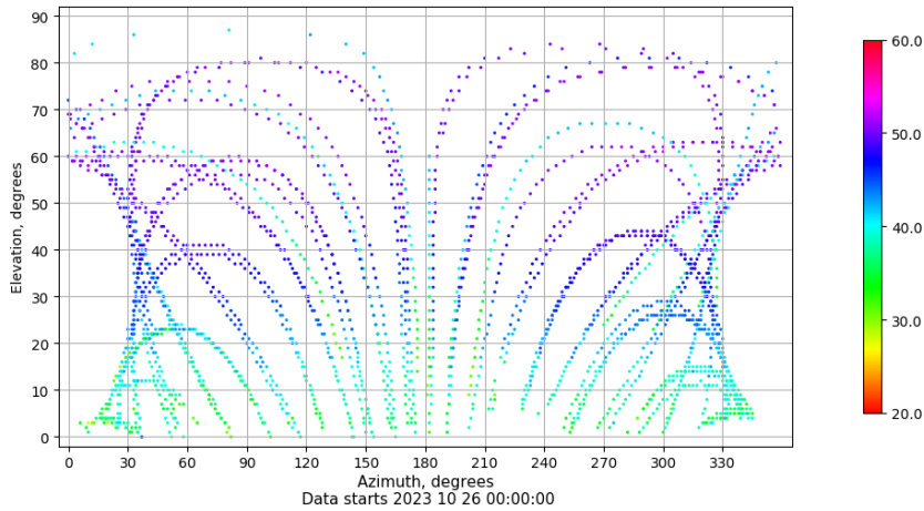
Azimuth-elevation plot for station BCL1. Signal to Noise S1C Data file BCL100ESP_R_2023299.xtr
