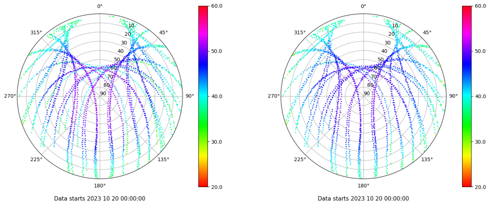
Skyplot for station BCL1. Signal to Noise S1C Data file BCL100ESP_R_2023293.xtr Skyplot for station BCL1. Signal to Noise S2P Data file BCL100ESP_R_2023293.xtr
