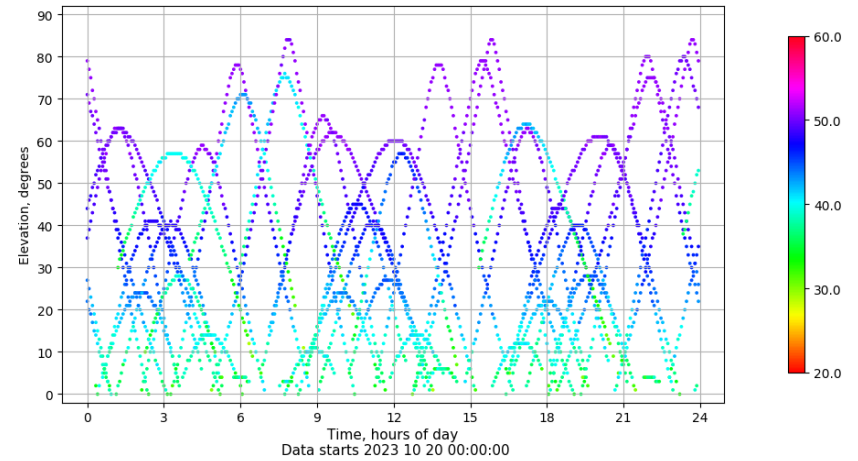
Time-elevation plot for station BCL1. Signal to Noise S1C Data file BCL100ESP_R_2023293.xtr
