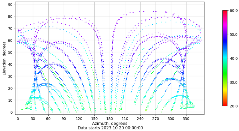
Azimuth-elevation plot for station BCL1. Signal to Noise S1C Data file BCL100ESP_R_2023293.xtr
