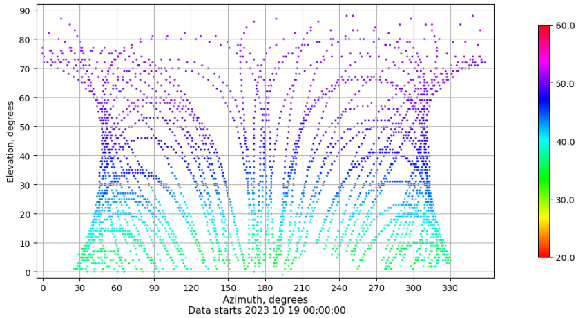
Azimuth-elevation plot for station BCL1. Signal to Noise S1C Data file BCL100ESP_R_2023292.xtr
