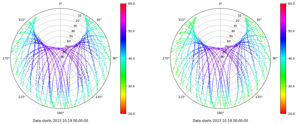
Skyplot for station BCL1. Signal to Noise S1C Data file BCL100ESP_R_2023292.xtr Skyplot for station BCL1. Signal to Noise S2W Data file BCL100ESP_R_2023292.xtr
