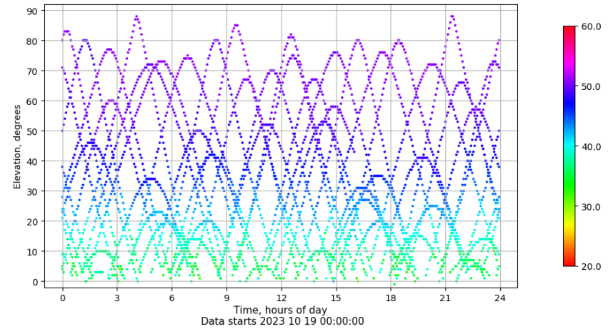
Time-elevation plot for station BCL1. Signal to Noise S1C Data file BCL100ESP_R_2023292.xtr
