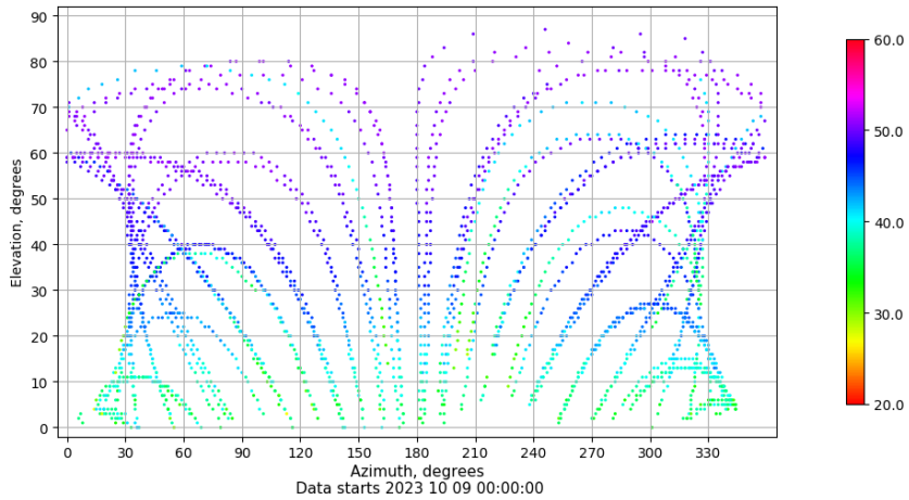
Azimuth-elevation plot for station BCL1. Signal to Noise S1C Data file BCL100ESP_R_2023282.xtr
