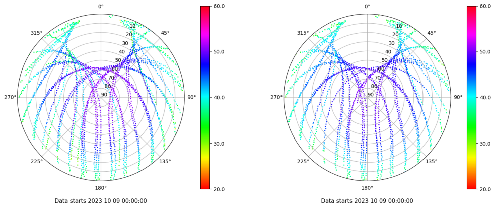
Skyplot for station BCL1. Signal to Noise S1C Data file BCL100ESP_R_2023282.xtr Skyplot for station BCL1. Signal to Noise S2P Data file BCL100ESP_R_2023282.xtr
