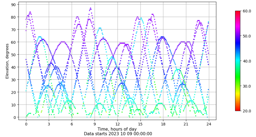
Time-elevation plot for station BCL1. Signal to Noise S1C Data file BCL100ESP_R_2023282.xtr
