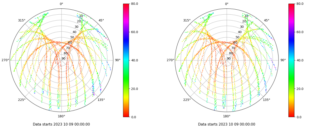
Skyplot for station BCL1. Parameter M1C Data file BCL100ESP_R_2023282.xtr Skyplot for station BCL1. Parameter M2P Data file BCL100ESP_R_2023282.xtr
