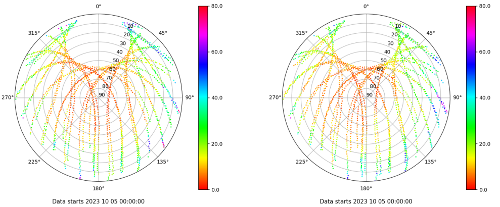
Skyplot for station BCL1. Parameter M1C Data file BCL100ESP_R_2023278.xtr Skyplot for station BCL1. Parameter M2P Data file BCL100ESP_R_2023278.xtr
