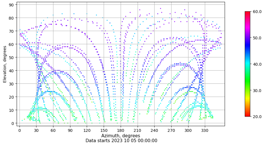
Azimuth-elevation plot for station BCL1. Signal to Noise S1C Data file BCL100ESP_R_2023278.xtr
