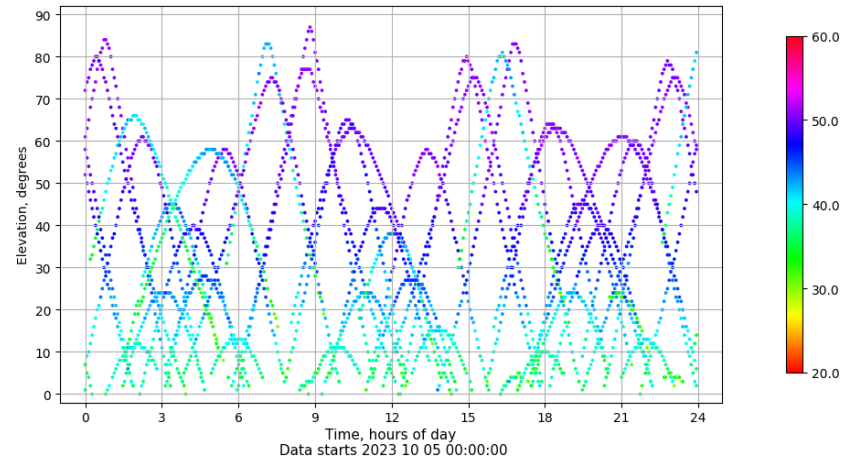
Time-elevation plot for station BCL1. Signal to Noise S1C Data file BCL100ESP_R_2023278.xtr
