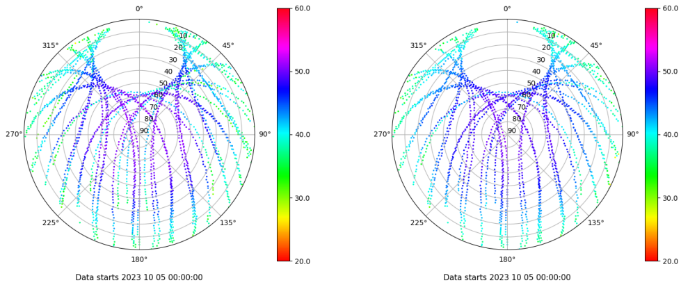
Skyplot for station BCL1. Signal to Noise S1C Data file BCL100ESP_R_2023278.xtr Skyplot for station BCL1. Signal to Noise S2P Data file BCL100ESP_R_2023278.xtr
