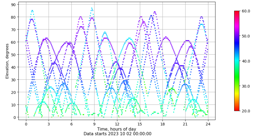
Time-elevation plot for station BCL1. Signal to Noise S1C Data file BCL100ESP_R_2023275.xtr
