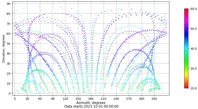
Azimuth-elevation plot for station BCL1. Signal to Noise S1C Data file BCL100ESP_R_2023275.xtr
