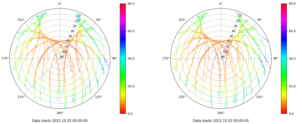
Skyplot for station BCL1. Parameter M1C Data file BCL100ESP_R_2023275.xtr Skyplot for station BCL1. Parameter M2P Data file BCL100ESP_R_2023275.xtr
