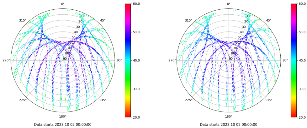
Skyplot for station BCL1. Signal to Noise S1C Data file BCL100ESP_R_2023275.xtr Skyplot for station BCL1. Signal to Noise S2P Data file BCL100ESP_R_2023275.xtr
