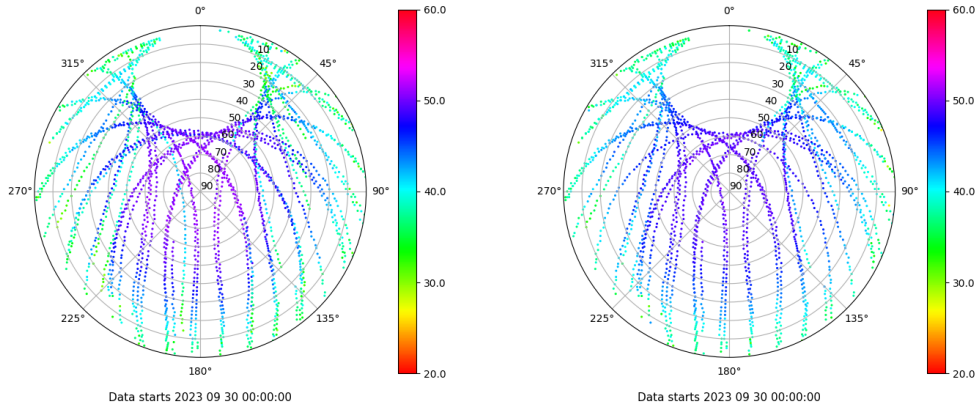
Skyplot for station BCL1. Signal to Noise S1C Data file BCL100ESP_R_2023273.xtr Skyplot for station BCL1. Signal to Noise S2P Data file BCL100ESP_R_2023273.xtr
