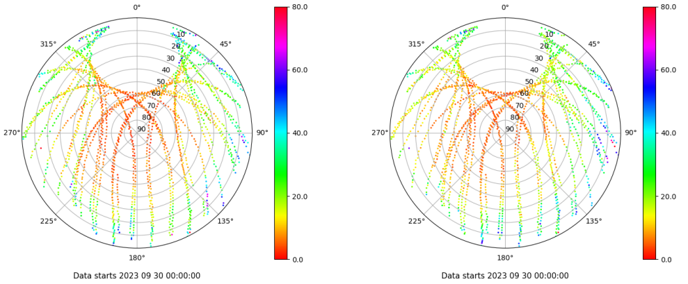
Skyplot for station BCL1. Parameter M1C Data file BCL100ESP_R_2023273.xtr Skyplot for station BCL1. Parameter M2P Data file BCL100ESP_R_2023273.xtr
