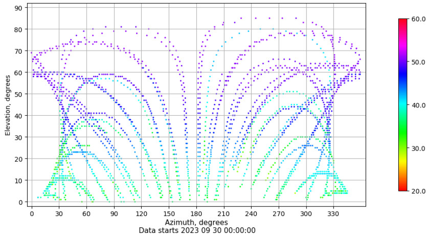
Azimuth-elevation plot for station BCL1. Signal to Noise S1C Data file BCL100ESP_R_2023273.xtr
