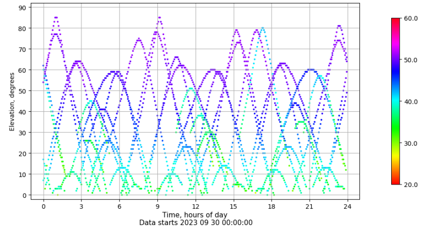
Time-elevation plot for station BCL1. Signal to Noise S1C Data file BCL100ESP_R_2023273.xtr
