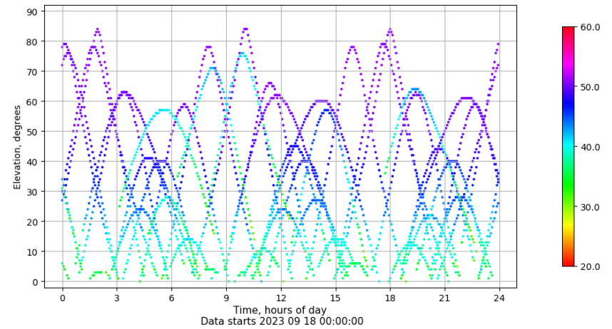
Time-elevation plot for station BCL1. Signal to Noise S1C Data file BCL100ESP_R_2023261.xtr
