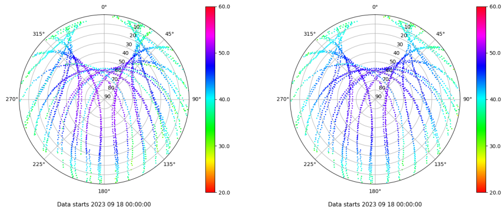
Skyplot for station BCL1. Signal to Noise S1C Data file BCL100ESP_R_2023261.xtr Skyplot for station BCL1. Signal to Noise S2P Data file BCL100ESP_R_2023261.xtr
