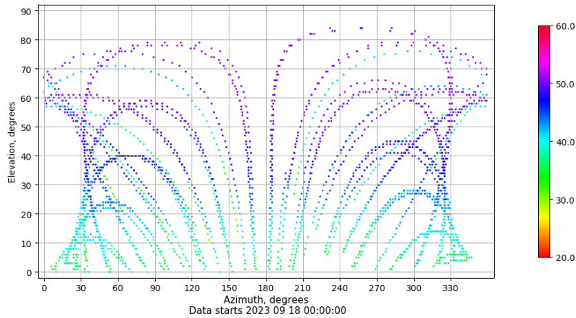
Azimuth-elevation plot for station BCL1. Signal to Noise S1C Data file BCL100ESP_R_2023261.xtr
