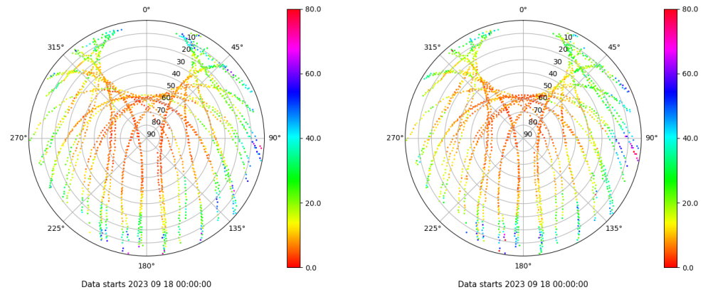
Skyplot for station BCL1. Parameter M1C Data file BCL100ESP_R_2023261.xtr Skyplot for station BCL1. Parameter M2P Data file BCL100ESP_R_2023261.xtr
