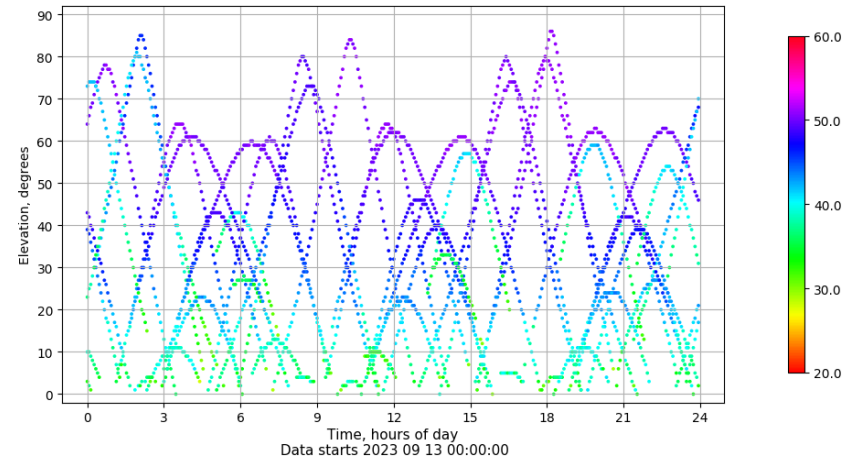
Time-elevation plot for station BCL1. Signal to Noise S1C Data file BCL100ESP_R_2023256.xtr
