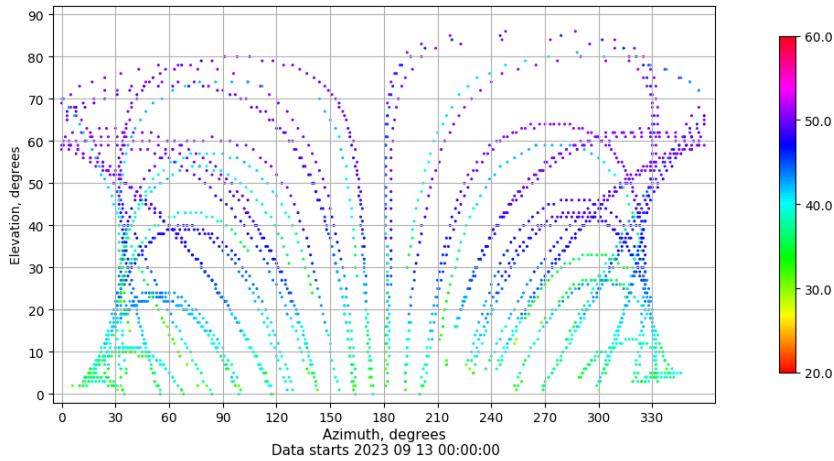
Azimuth-elevation plot for station BCL1. Signal to Noise S1C Data file BCL100ESP_R_2023256.xtr
