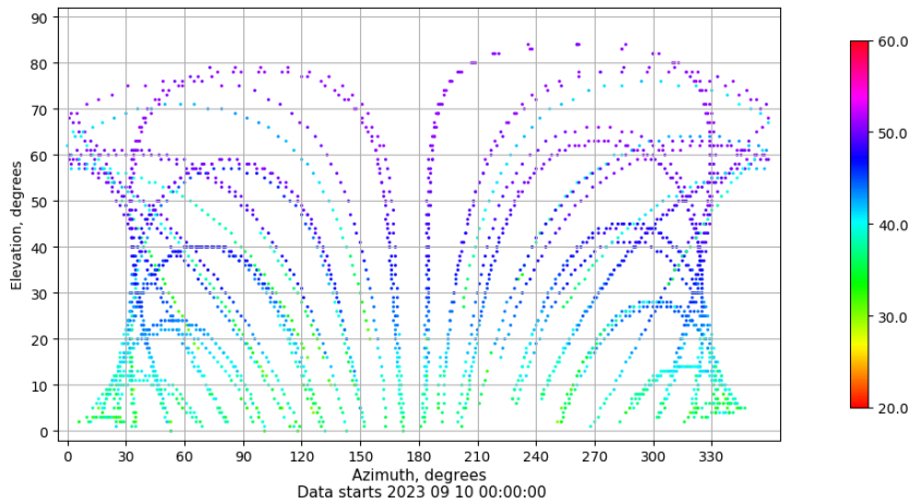
Azimuth-elevation plot for station BCL1. Signal to Noise S1C Data file BCL100ESP_R_2023253.xtr
