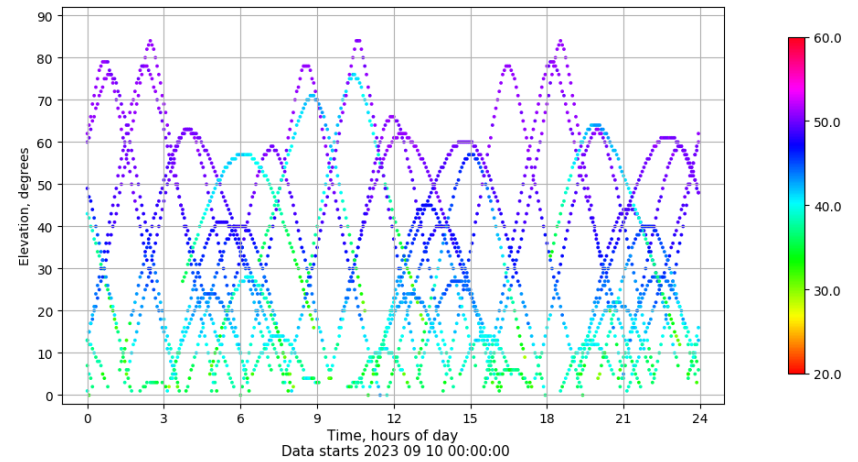
Time-elevation plot for station BCL1. Signal to Noise S1C Data file BCL100ESP_R_2023253.xtr
