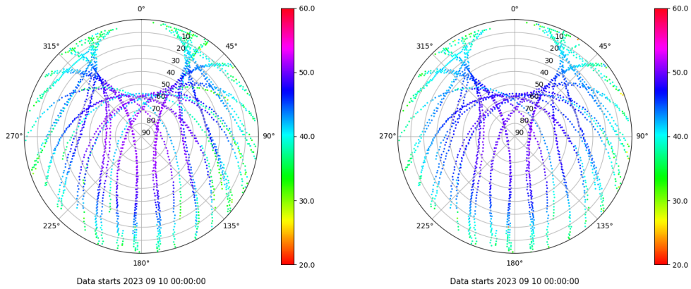
Skyplot for station BCL1. Signal to Noise S1C Data file BCL100ESP_R_2023253.xtr Skyplot for station BCL1. Signal to Noise S2P Data file BCL100ESP_R_2023253.xtr
