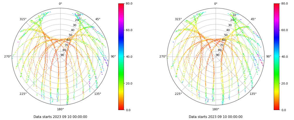
Skyplot for station BCL1. Parameter M1C Data file BCL100ESP_R_2023253.xtr Skyplot for station BCL1. Parameter M2P Data file BCL100ESP_R_2023253.xtr
