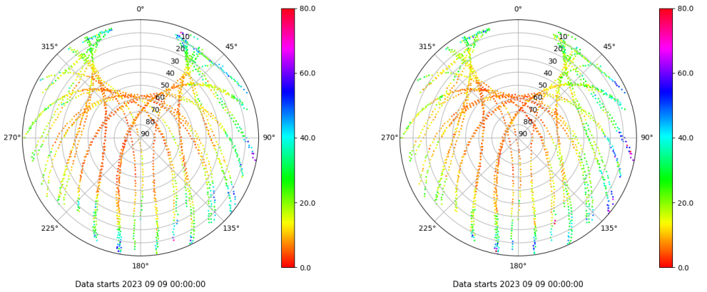
Skyplot for station BCL1. Parameter M1C Data file BCL100ESP_R_2023252.xtr Skyplot for station BCL1. Parameter M2P Data file BCL100ESP_R_2023252.xtr
