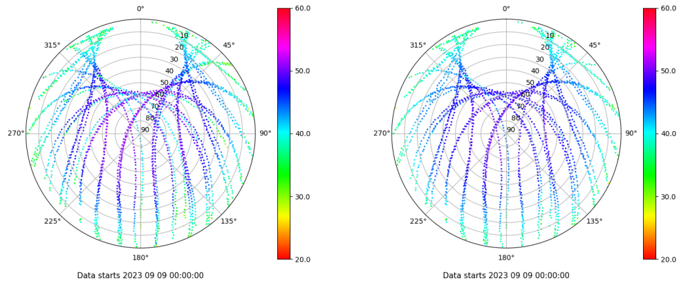
Skyplot for station BCL1. Signal to Noise S1C Data file BCL100ESP_R_2023252.xtr Skyplot for station BCL1. Signal to Noise S2P Data file BCL100ESP_R_2023252.xtr
