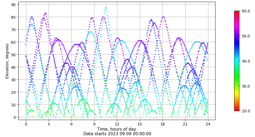
Time-elevation plot for station BCL1. Signal to Noise S1C Data file BCL100ESP_R_2023252.xtr
