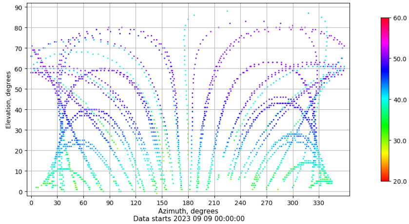
Azimuth-elevation plot for station BCL1. Signal to Noise S1C Data file BCL100ESP_R_2023252.xtr
