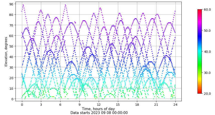
Time-elevation plot for station BCL1. Signal to Noise S1C Data file BCL100ESP_R_2023251.xtr
