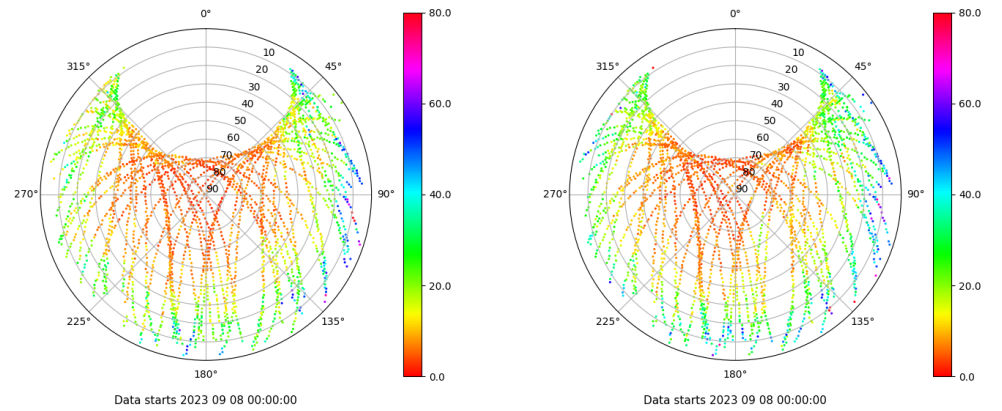
Skyplot for station BCL1. Parameter M1C Data file BCL100ESP_R_2023251.xtr Skyplot for station BCL1. Parameter M2W Data file BCL100ESP_R_2023251.xtr
