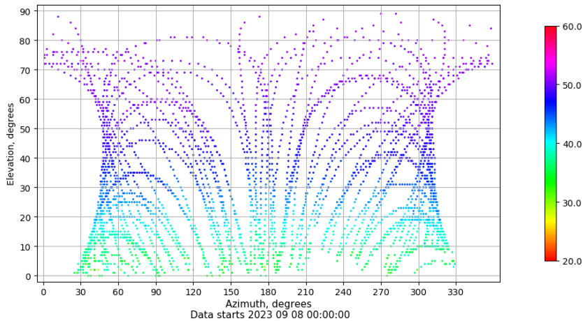
Azimuth-elevation plot for station BCL1. Signal to Noise S1C Data file BCL100ESP_R_2023251.xtr
