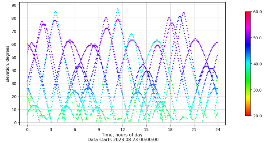
Time-elevation plot for station BCL1. Signal to Noise S1C Data file BCL100ESP_R_2023235.xtr
