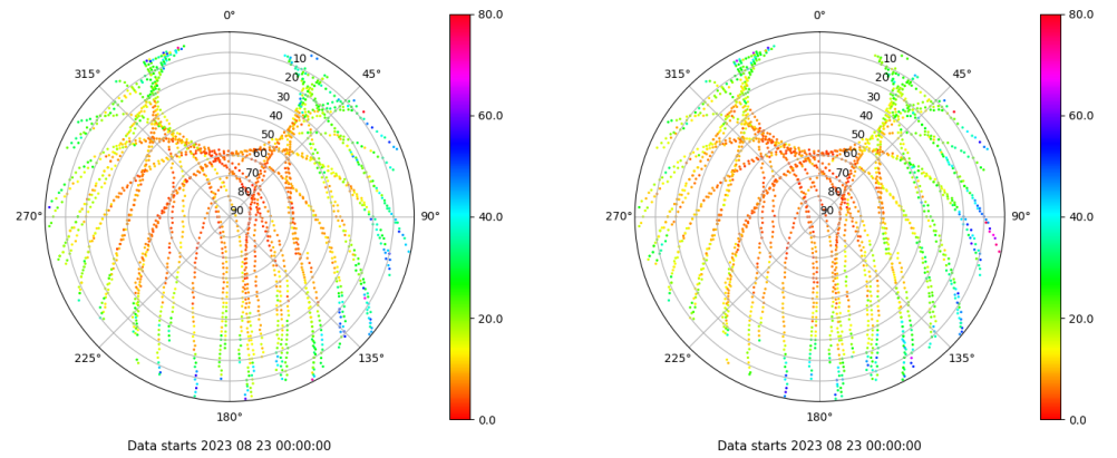
Skyplot for station BCL1. Parameter M1C Data file BCL100ESP_R_2023235.xtr Skyplot for station BCL1. Parameter M2P Data file BCL100ESP_R_2023235.xtr
