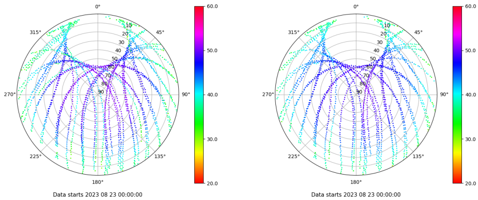
Skyplot for station BCL1. Signal to Noise S1C Data file BCL100ESP_R_2023235.xtr Skyplot for station BCL1. Signal to Noise S2P Data file BCL100ESP_R_2023235.xtr
