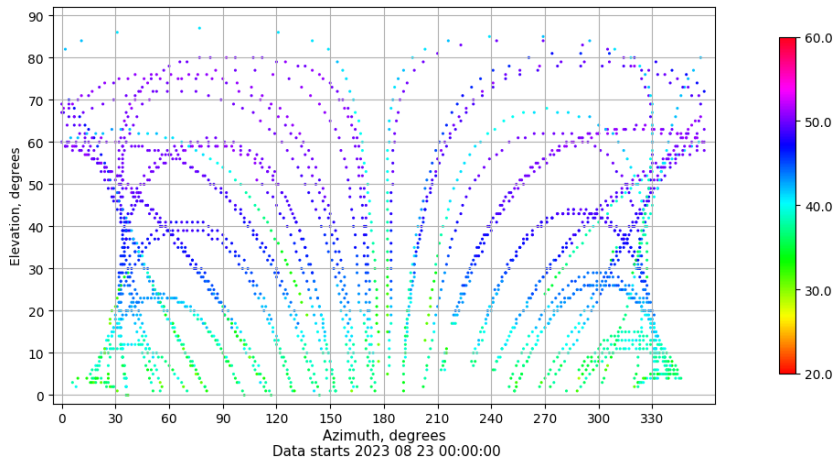
Azimuth-elevation plot for station BCL1. Signal to Noise S1C Data file BCL100ESP_R_2023235.xtr
