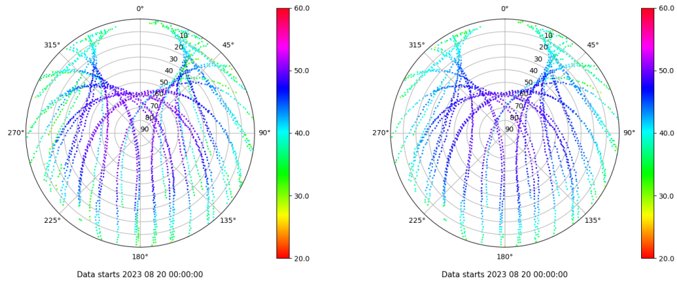
Skyplot for station BCL1. Signal to Noise S1C Data file BCL100ESP_R_2023232.xtr Skyplot for station BCL1. Signal to Noise S2P Data file BCL100ESP_R_2023232.xtr
