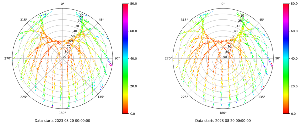
Skyplot for station BCL1. Parameter M1C Data file BCL100ESP_R_2023232.xtr Skyplot for station BCL1. Parameter M2P Data file BCL100ESP_R_2023232.xtr
