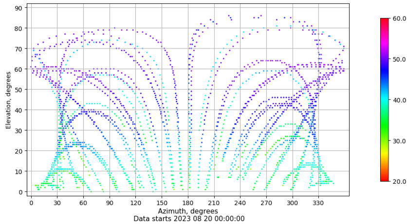
Azimuth-elevation plot for station BCL1. Signal to Noise S1C Data file BCL100ESP_R_2023232.xtr
