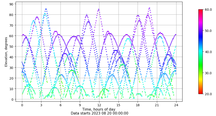
Time-elevation plot for station BCL1. Signal to Noise S1C Data file BCL100ESP_R_2023232.xtr
