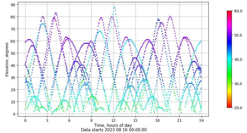
Time-elevation plot for station BCL1. Signal to Noise S1C Data file BCL100ESP_R_2023228.xtr
