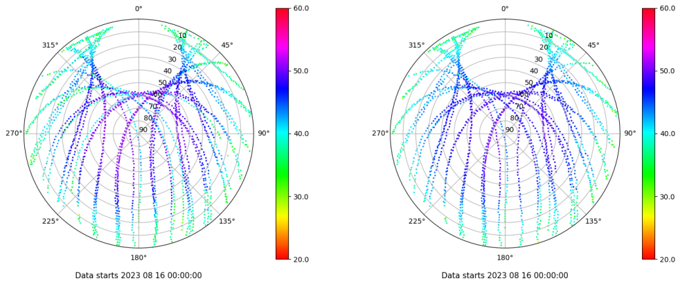
Skyplot for station BCL1. Signal to Noise S1C Data file BCL100ESP_R_2023228.xtr Skyplot for station BCL1. Signal to Noise S2P Data file BCL100ESP_R_2023228.xtr
