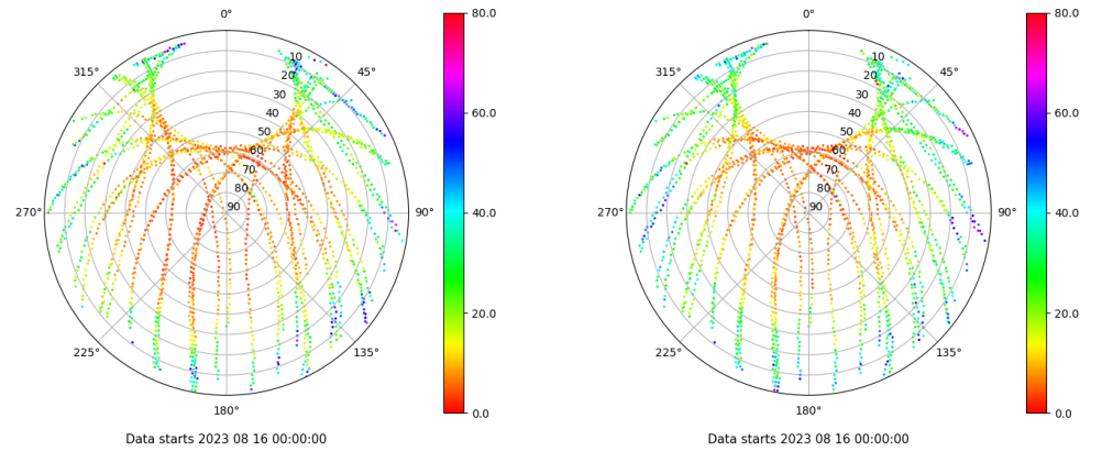
Skyplot for station BCL1. Parameter M1C Data file BCL100ESP_R_2023228.xtr Skyplot for station BCL1. Parameter M2P Data file BCL100ESP_R_2023228.xtr
