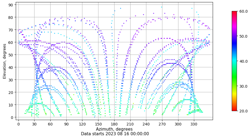
Azimuth-elevation plot for station BCL1. Signal to Noise S1C Data file BCL100ESP_R_2023228.xtr
