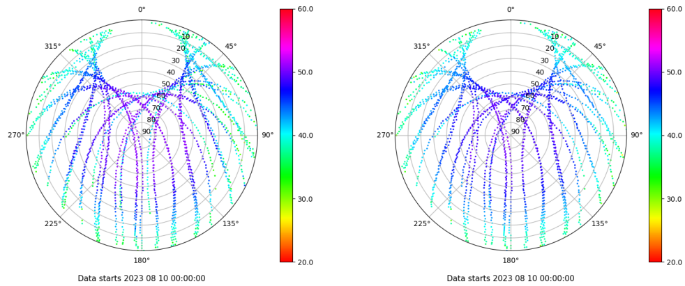
Skyplot for station BCL1. Signal to Noise S1C Data file BCL100ESP_R_2023222.xtr Skyplot for station BCL1. Signal to Noise S2P Data file BCL100ESP_R_2023222.xtr
