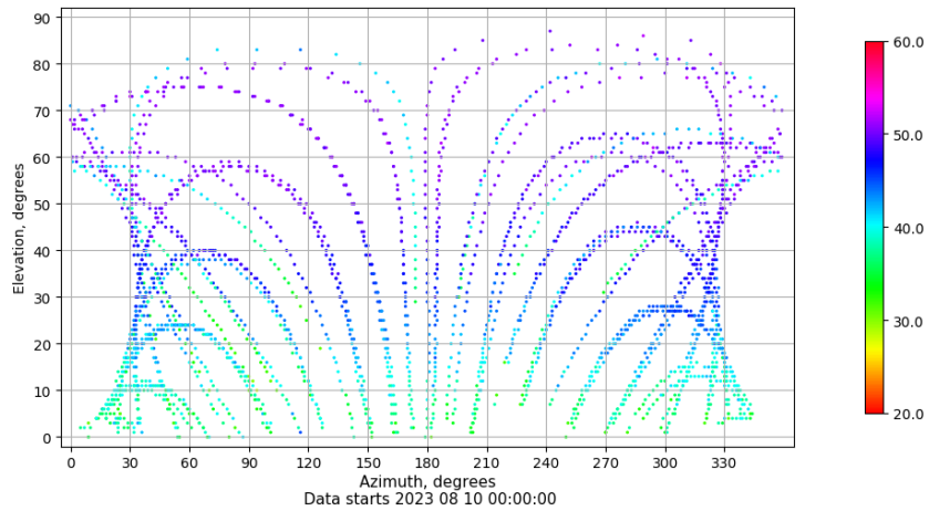
Azimuth-elevation plot for station BCL1. Signal to Noise S1C Data file BCL100ESP_R_2023222.xtr
