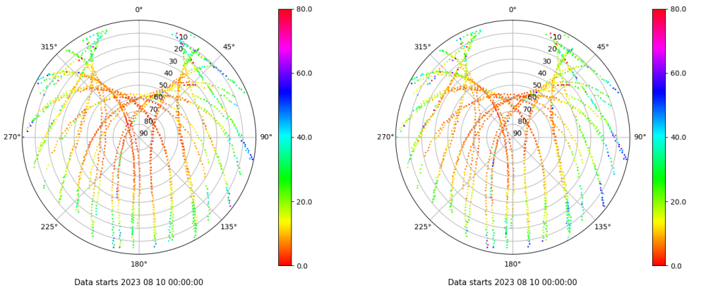
Skyplot for station BCL1. Parameter M1C Data file BCL100ESP_R_2023222.xtr Skyplot for station BCL1. Parameter M2P Data file BCL100ESP_R_2023222.xtr
