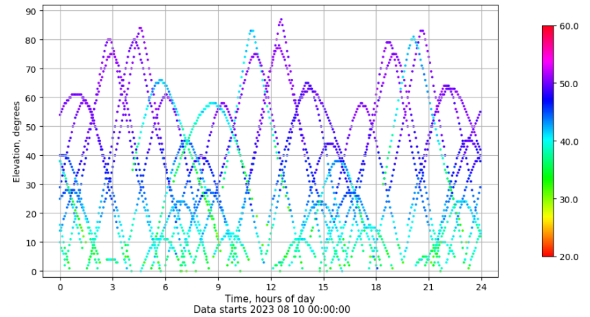
Time-elevation plot for station BCL1. Signal to Noise S1C Data file BCL100ESP_R_2023222.xtr
