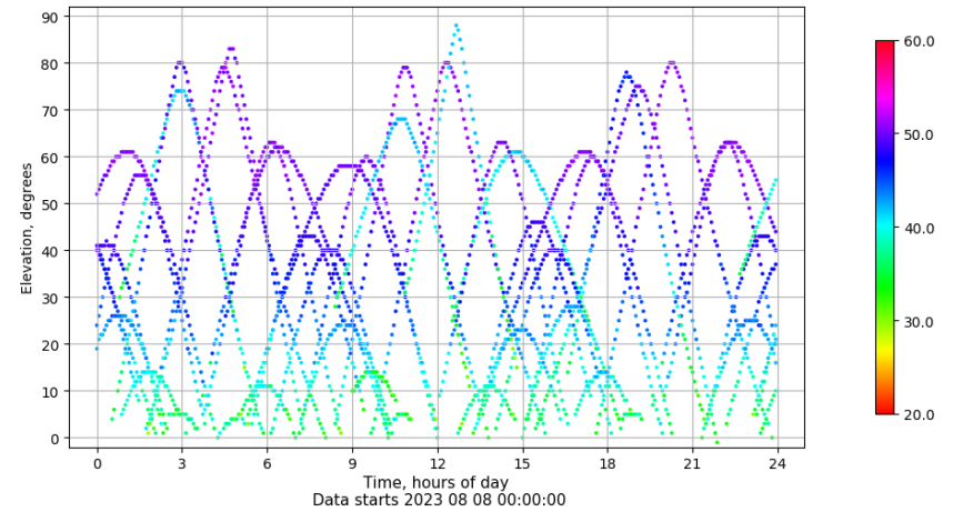
Time-elevation plot for station BCL1. Signal to Noise S1C Data file BCL100ESP_R_2023220.xtr
