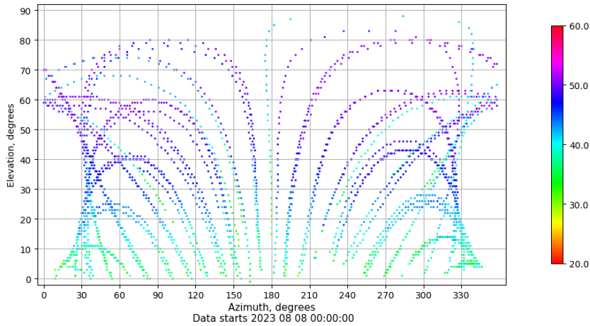
Azimuth-elevation plot for station BCL1. Signal to Noise S1C Data file BCL100ESP_R_2023220.xtr
