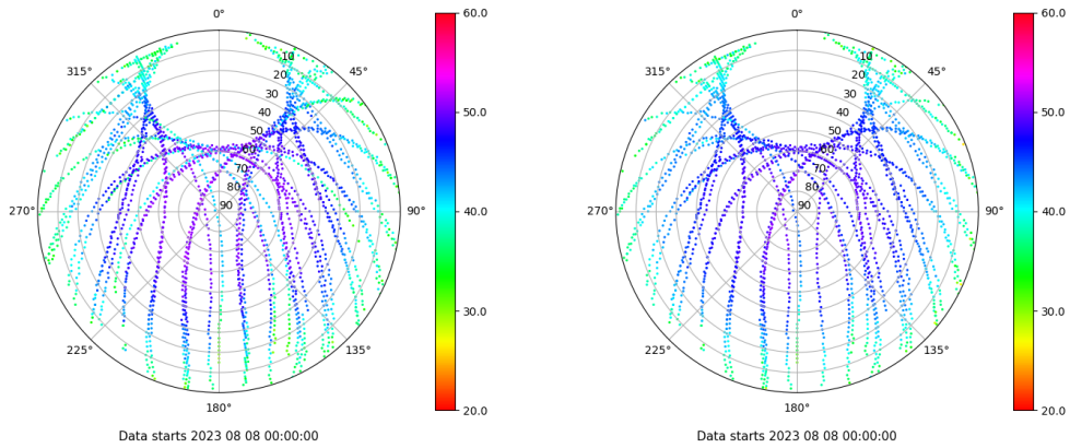
Skyplot for station BCL1. Signal to Noise S1C Data file BCL100ESP_R_2023220.xtr Skyplot for station BCL1. Signal to Noise S2P Data file BCL100ESP_R_2023220.xtr
