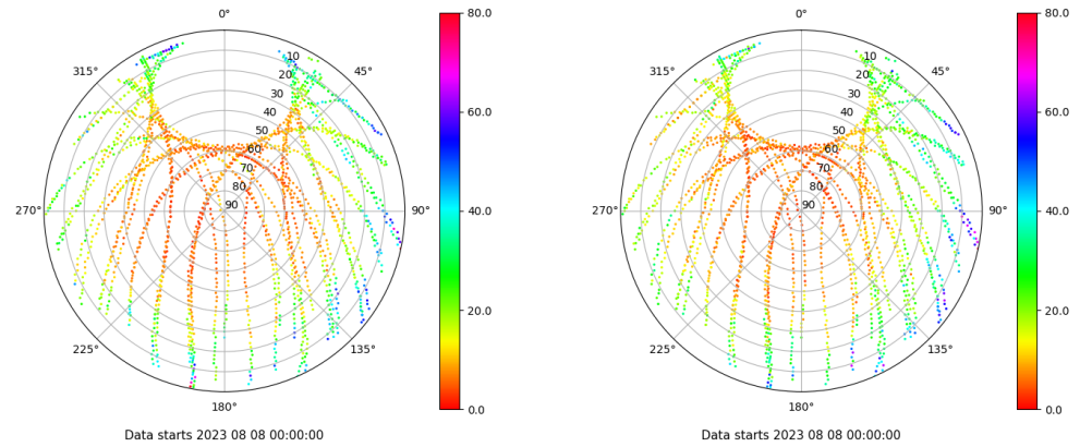
Skyplot for station BCL1. Parameter M1C Data file BCL100ESP_R_2023220.xtr Skyplot for station BCL1. Parameter M2P Data file BCL100ESP_R_2023220.xtr
