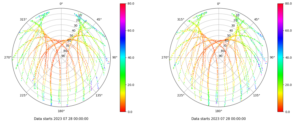
Skyplot for station BCL1. Parameter M1C Data file BCL100ESP_R_2023209.xtr Skyplot for station BCL1. Parameter M2P Data file BCL100ESP_R_2023209.xtr
