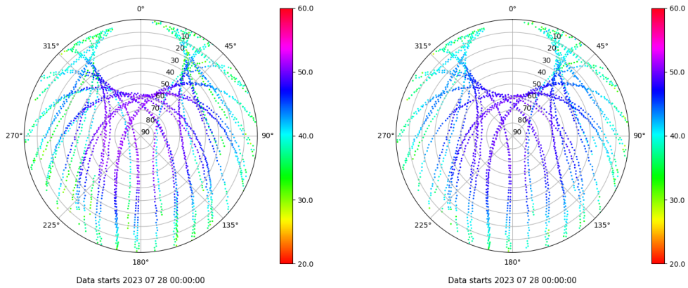
Skyplot for station BCL1. Signal to Noise S1C Data file BCL100ESP_R_2023209.xtr Skyplot for station BCL1. Signal to Noise S2P Data file BCL100ESP_R_2023209.xtr
