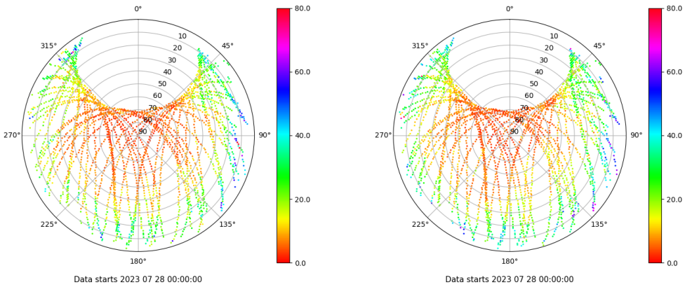
Skyplot for station BCL1. Parameter M1C Data file BCL100ESP_R_2023209.xtr Skyplot for station BCL1. Parameter M2W Data file BCL100ESP_R_2023209.xtr
