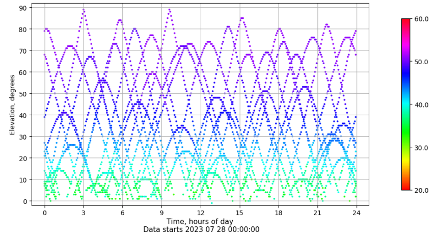
Time-elevation plot for station BCL1. Signal to Noise S1C Data file BCL100ESP_R_2023209.xtr
