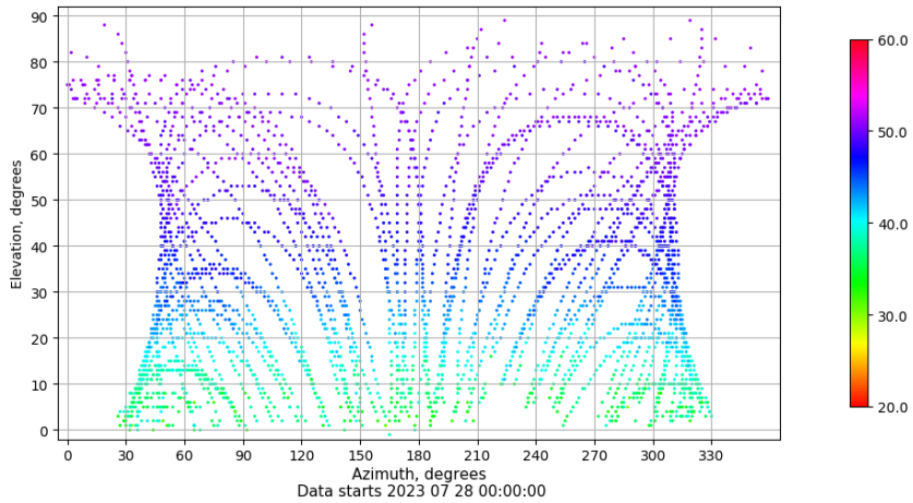
Azimuth-elevation plot for station BCL1. Signal to Noise S1C Data file BCL100ESP_R_2023209.xtr
