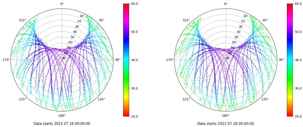
Skyplot for station BCL1. Signal to Noise S1C Data file BCL100ESP_R_2023209.xtr Skyplot for station BCL1. Signal to Noise S2W Data file BCL100ESP_R_2023209.xtr
