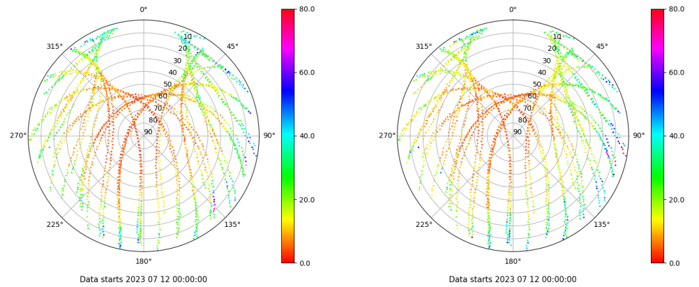
Skyplot for station BCL1. Parameter M1C Data file BCL100ESP_R_2023193.xtr Skyplot for station BCL1. Parameter M2P Data file BCL100ESP_R_2023193.xtr
