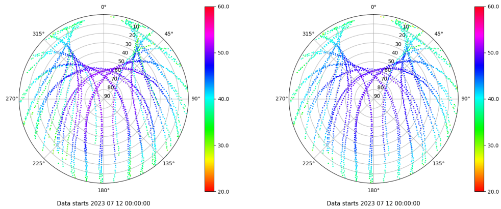
Skyplot for station BCL1. Signal to Noise S1C Data file BCL100ESP_R_2023193.xtr Skyplot for station BCL1. Signal to Noise S2P Data file BCL100ESP_R_2023193.xtr
