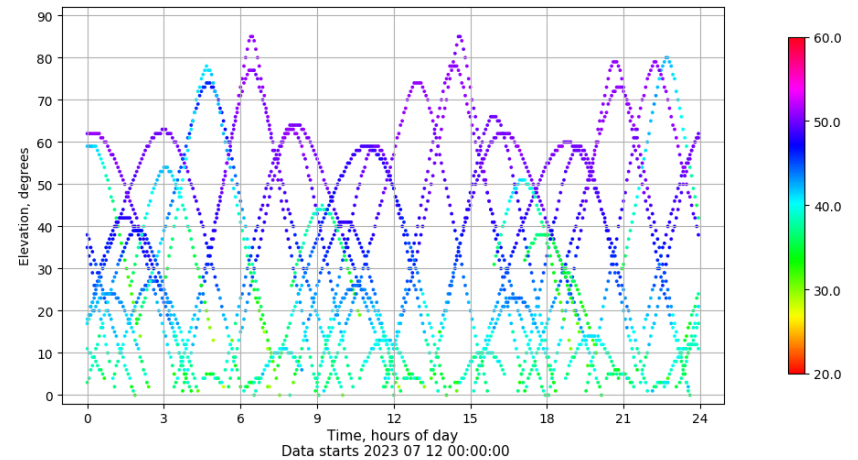
Time-elevation plot for station BCL1. Signal to Noise S1C Data file BCL100ESP_R_2023193.xtr
