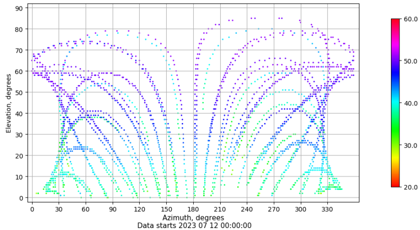
Azimuth-elevation plot for station BCL1. Signal to Noise S1C Data file BCL100ESP_R_2023193.xtr
