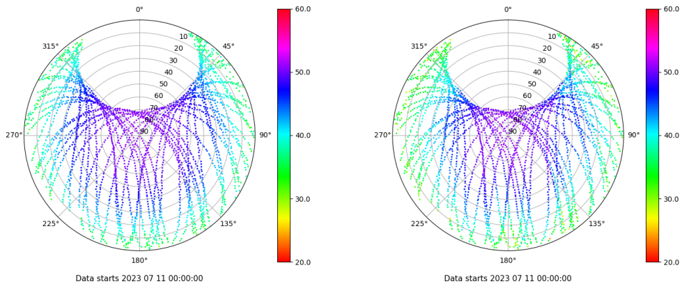
Skyplot for station BCL1. Signal to Noise S1C Data file BCL100ESP_R_2023192.xtr Skyplot for station BCL1. Signal to Noise S2W Data file BCL100ESP_R_2023192.xtr
