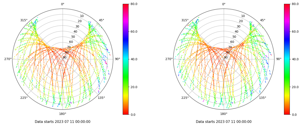
Skyplot for station BCL1. Parameter M1C Data file BCL100ESP_R_2023192.xtr Skyplot for station BCL1. Parameter M2W Data file BCL100ESP_R_2023192.xtr
