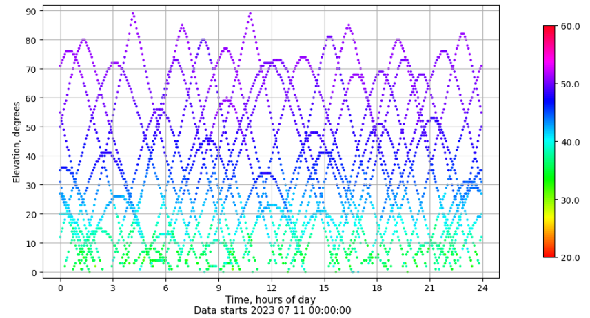
Time-elevation plot for station BCL1. Signal to Noise S1C Data file BCL100ESP_R_2023192.xtr
