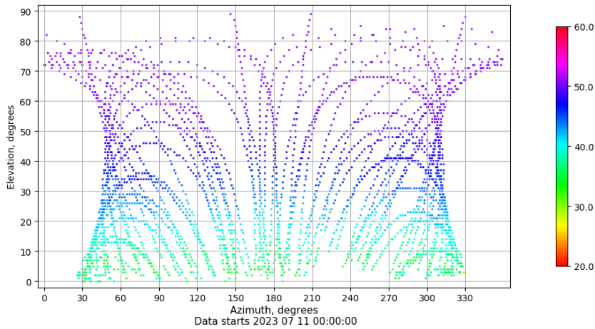
Azimuth-elevation plot for station BCL1. Signal to Noise S1C Data file BCL100ESP_R_2023192.xtr
